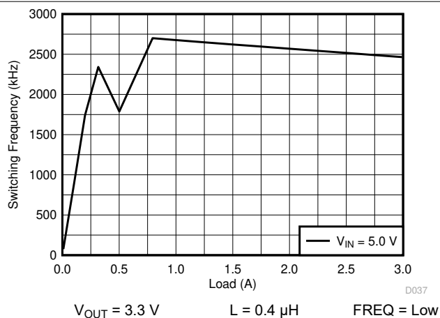
5-10. Frequency vs Load Current
