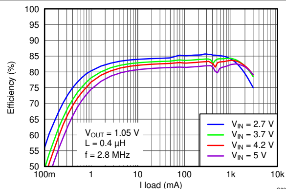
Figure 7-7. Efficiency vs Load Current
