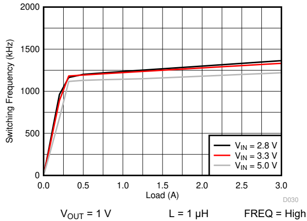
図 5-3. Switching Frequency vs Load Current
