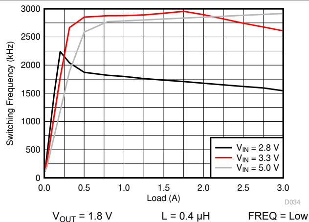
5-7. Frequency vs Load Current
