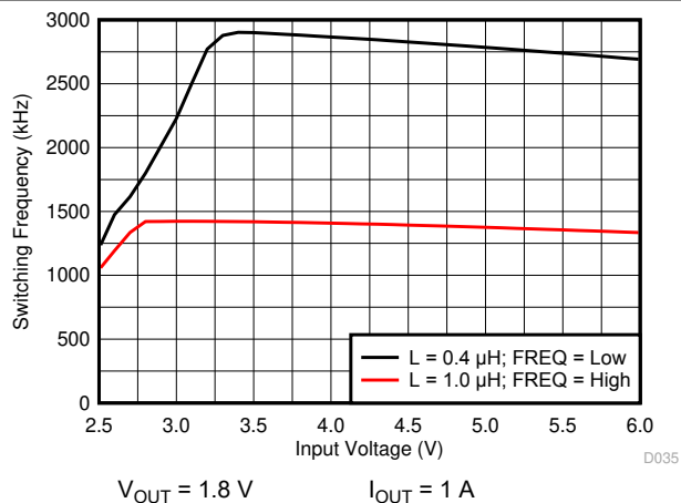
5-8. Frequency vs Input Voltage
