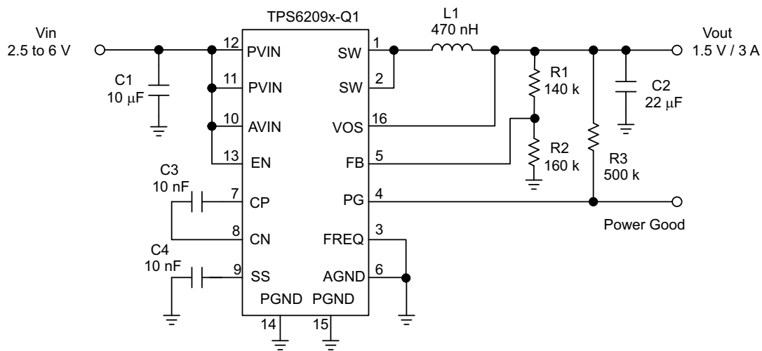
図 7-22. 1.5-V Adjustable Version Operating at 2.8 MHz
