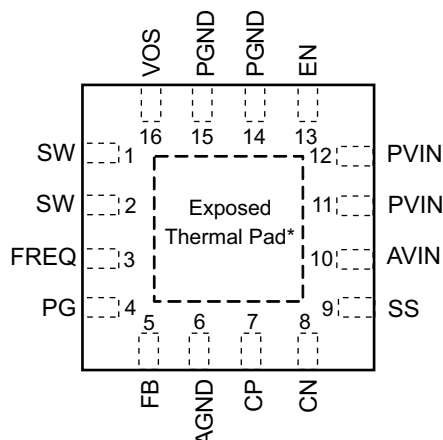
図 4-1. RGT Package 16-Pin QFN With Exposed Thermal Pad (Top View)
