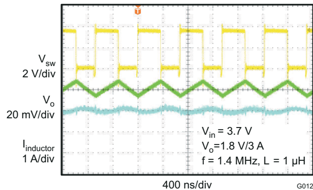
Figure 7-10. PWM Operation
