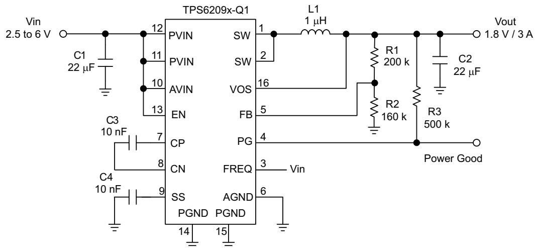
図 7-23. 1.8-V Adjustable Version Operating at 1.4 MHz
