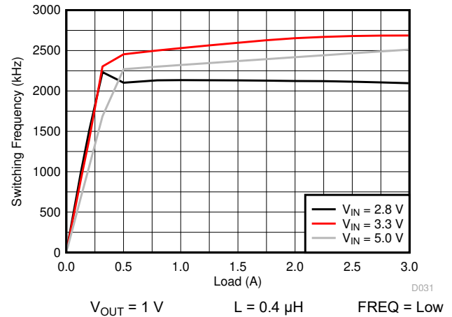
図 5-4. Switching Frequency vs Load Current
