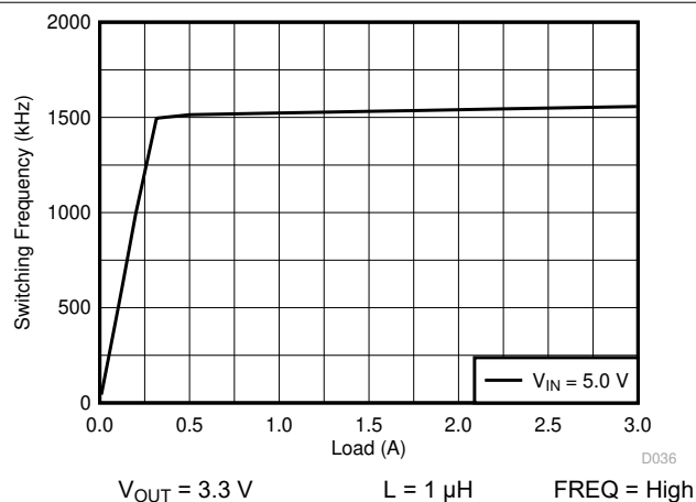
5-9. Frequency vs Load Current
