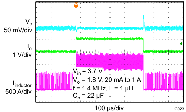
図 7-21. Load Transient Response
