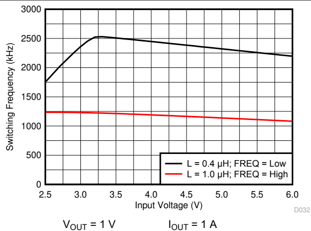
図 5-5. Frequency vs Input Voltage
