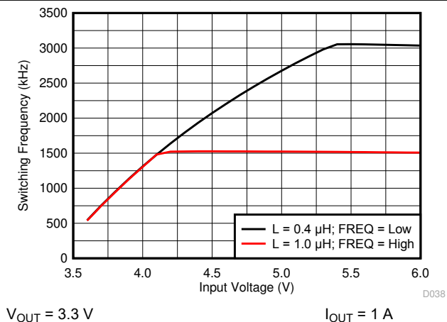
5-11. Frequency vs Input Voltage
