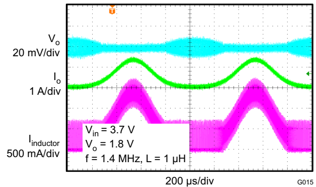
Figure 7-13. Load Sweep
