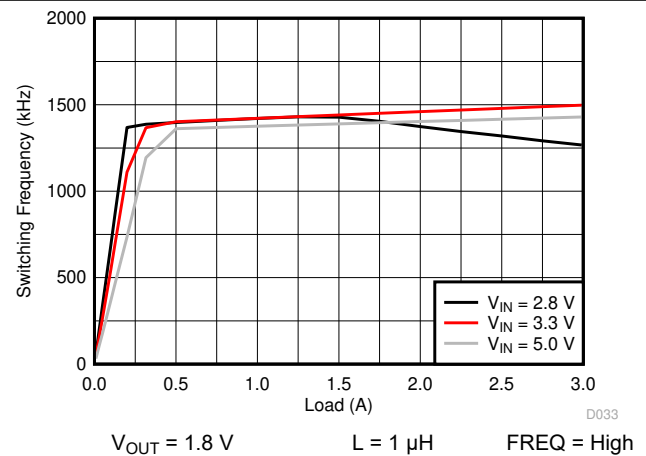
図 5-6. Frequency vs Load Current
