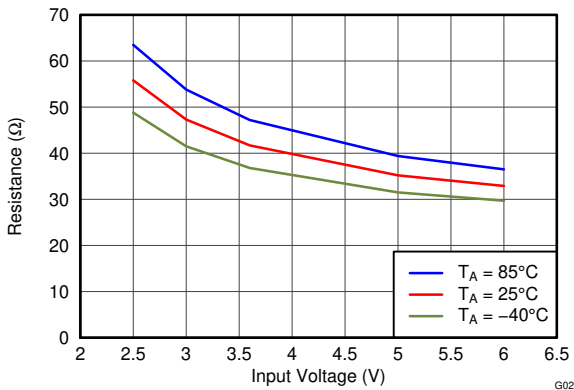
図 5-1. High-Side FET ON-Resistance vs Input Voltage
