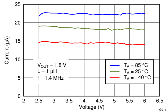
図 5-2. Quiescent Current vs Input Voltage
