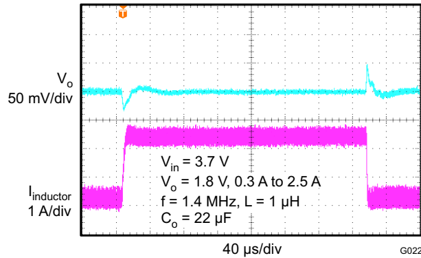
図 7-20. Load Transient Response
