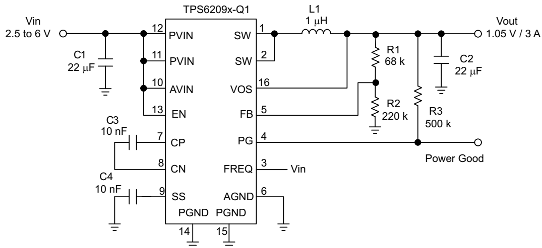
図 7-24. 1.05-V Adjustable Version Operating at 1.4 MHz
