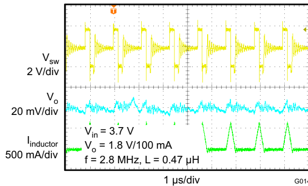
Figure 7-12. PFM Operation
