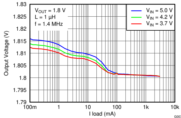
Figure 7-8. Output Voltage vs Load Current
