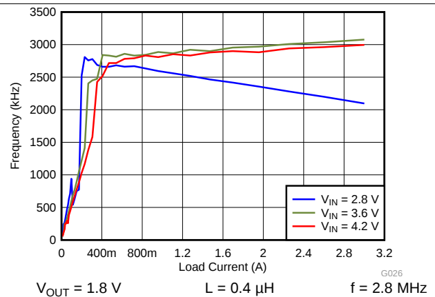
图 2. Switching Frequency vs Load Current
