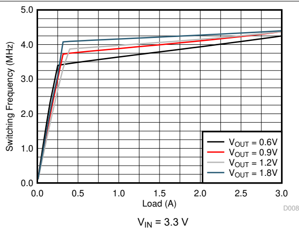
図 8-23. Switching Frequency
