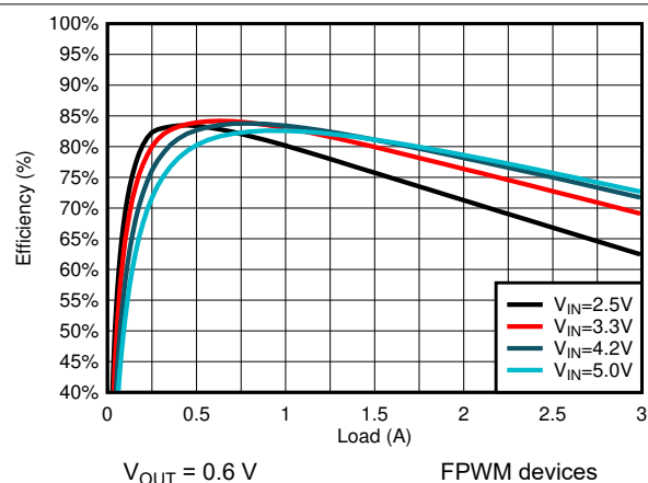
図 8-5. Efficiency
