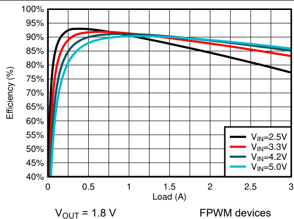
8-17. Efficiency
