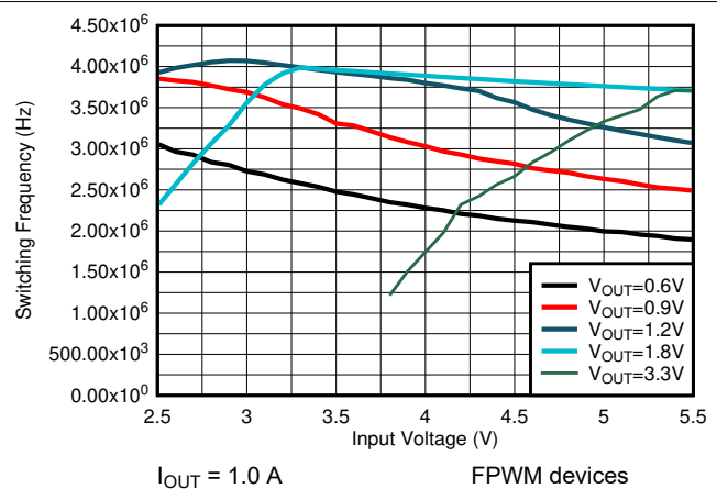
図 8-26. Switching Frequency
