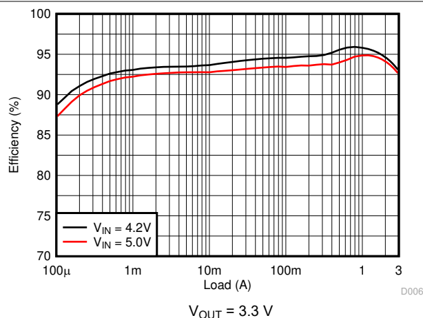
8-19. Efficiency
