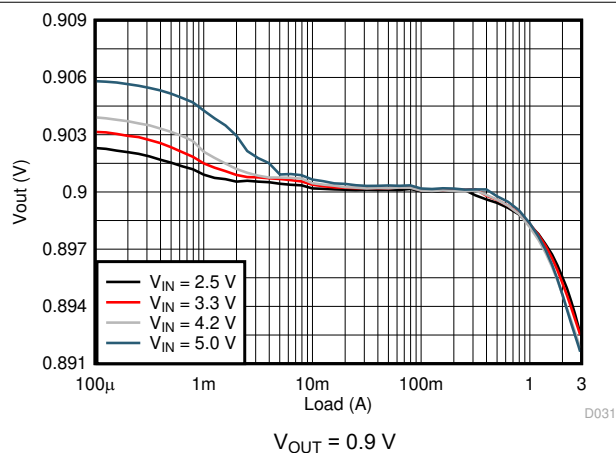
図 8-8. Load Regulation
