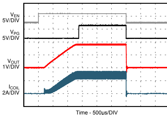
図 8-30. Start-Up With No Load
