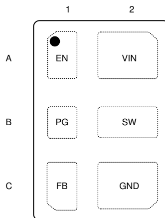
図 5-2. 6-Pin YWC Package, DSBGA (Top View)
