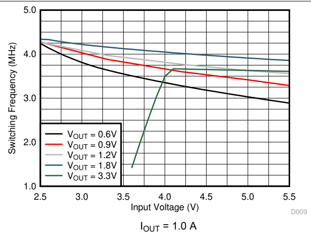
図 8-24. Switching Frequency
