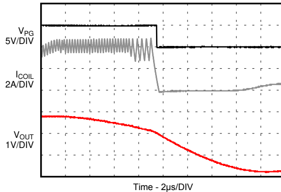
図 8-34. HICCUP Short-Circuit Protection
