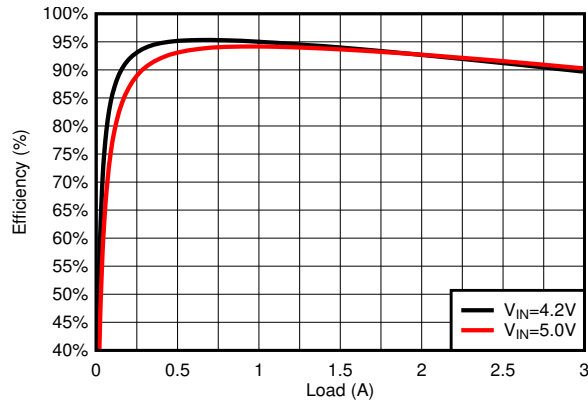
図 8-21. Efficiency
