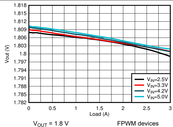
8-18. Load Regulation
