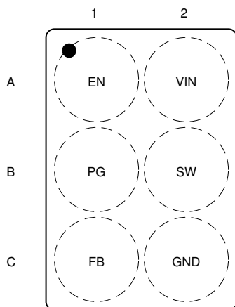
図 5-1. 6-Pin YFP Package, DSBGA (Top View)
