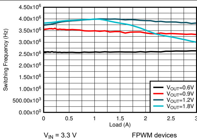
図 8-25. Switching Frequency
