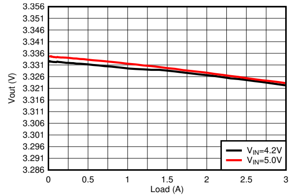
図 8-22. Load Regulation
