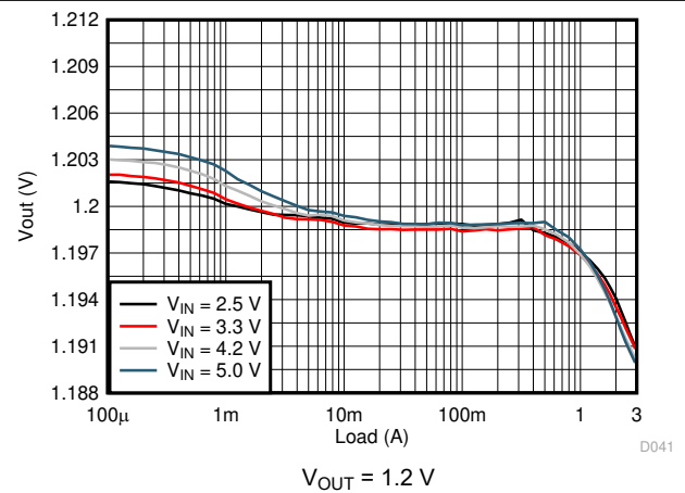
図 8-12. Load Regulation
