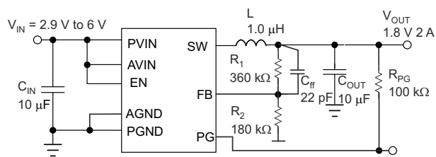
Typical Application Schematic
