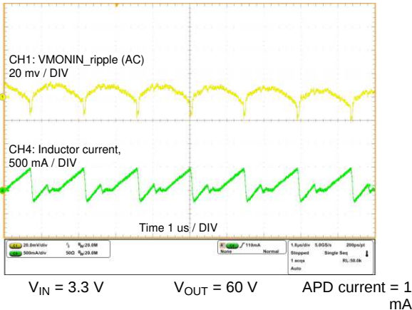
图 15. Output voltage ripple with 100 \Omega / 0.1 \mu\text{F} filter
