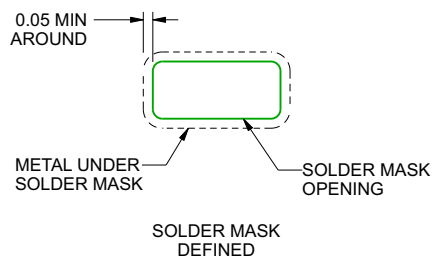
SOLDERMASK DETAILS
