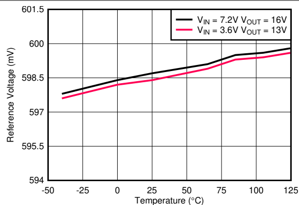
Figure 7-8. Reference Voltage vs Temperature
