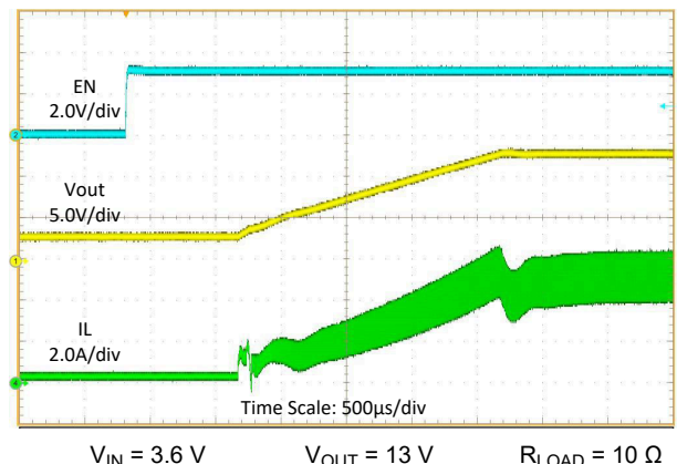
图 9-5. Start-up Waveforms
