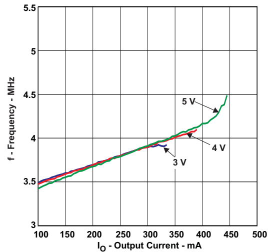
Figure 7. Frequency vs Output Load
