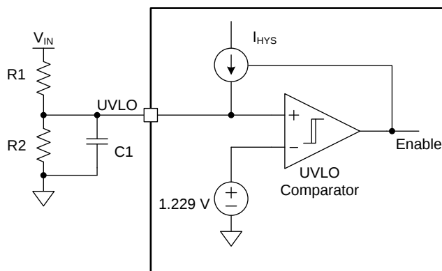
Figure 15. UVLO Circuit
