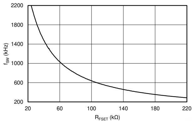
FIG 6-6. Boost Switching Frequency f_{SW} vs R_{FSET}
