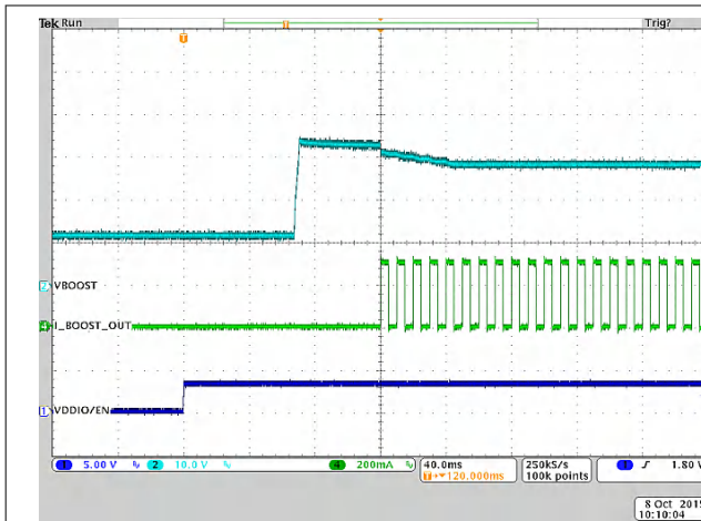
图 8-4. Typical Start-Up
