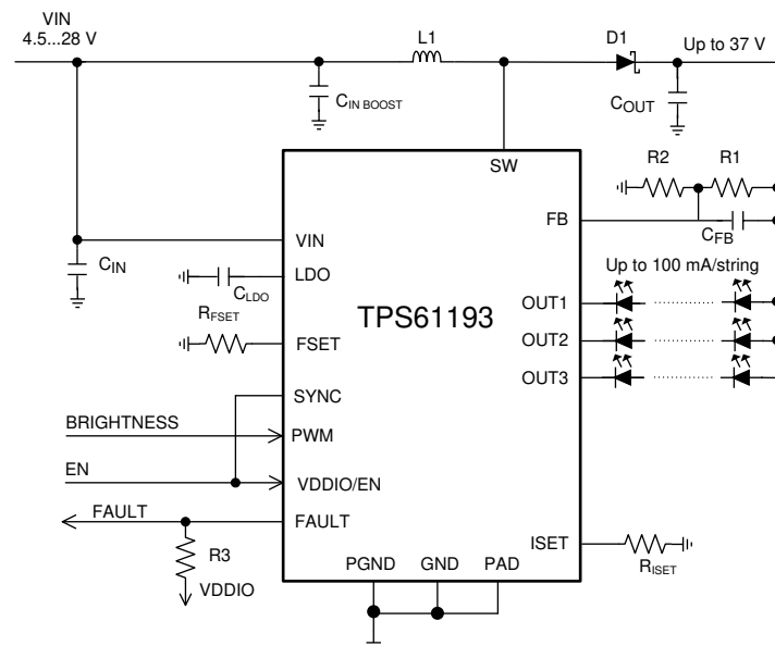
8-1. Three Strings 100-mA/String Configuration
