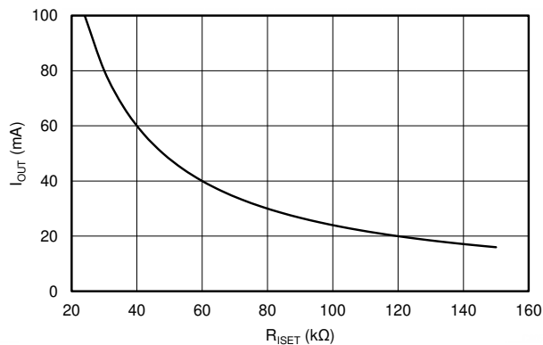
FIG 6-5. LED Current vs R_{ISET}
