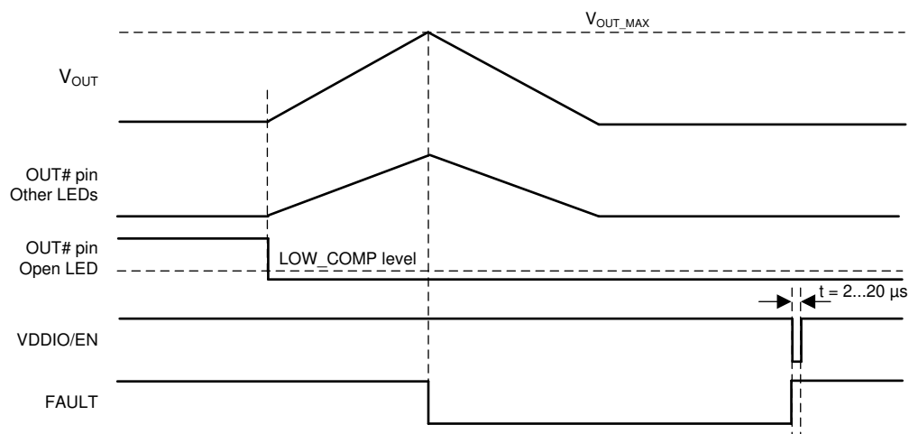
FIG 7-8. LED Open Fault
