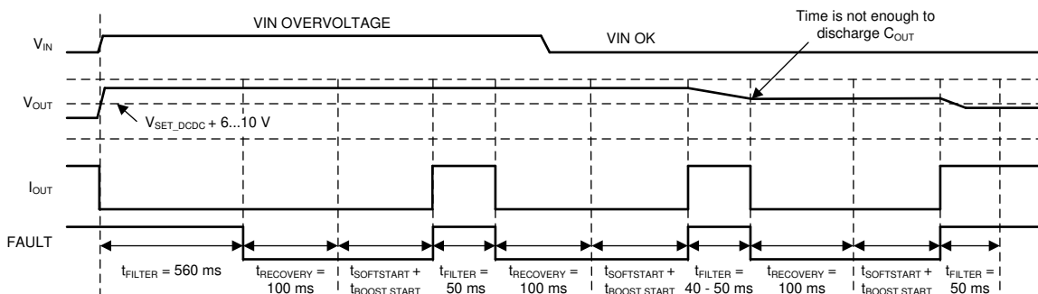
FIG 7-5. V_{IN} Overvoltage Protection (DC-DC OVP)
