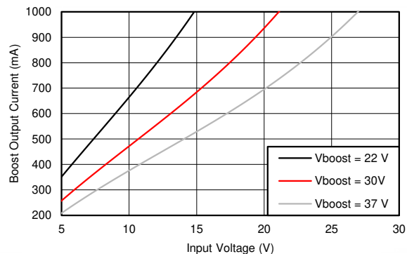
FIG 6-2. Maximum Boost Current
