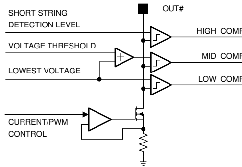
7-3. Comparators for Adaptive Voltage Control and LED Fault Detection
