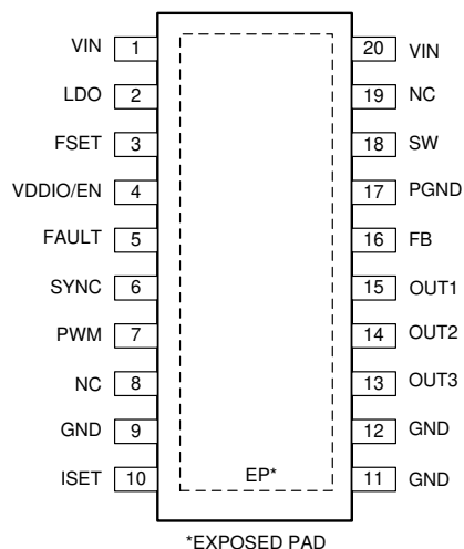
5-1. PWP Package 20-Pin TSSOP With Exposed Thermal Pad Top View
