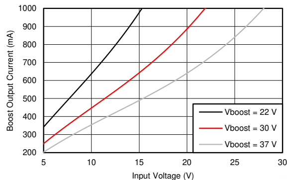
FIG 6-1. Maximum Boost Current
