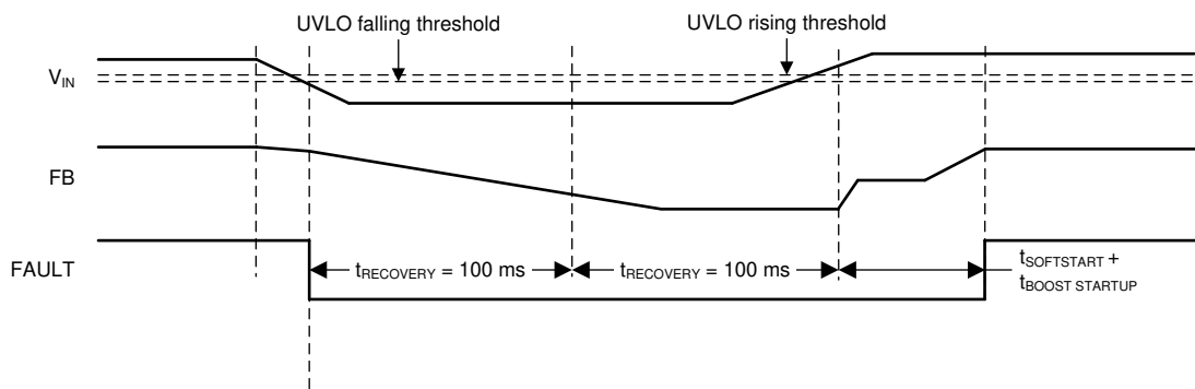
FIG 7-7. V_{IN} Undervoltage Lockout
