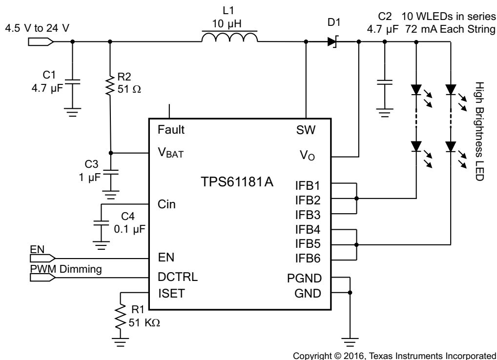
Figure 19. TPS61181A for Two Strings, High-Brightness LEDs Application
