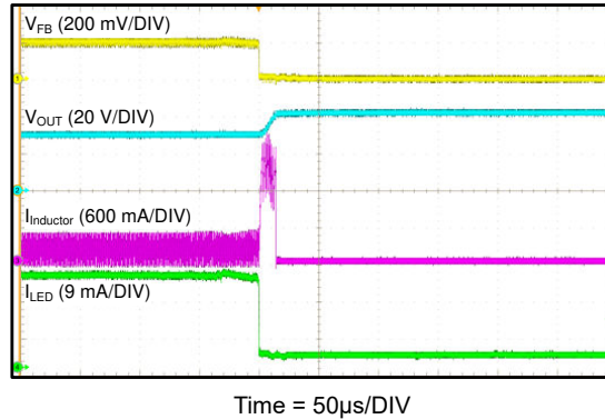
図 7-14. Open LED Protection
