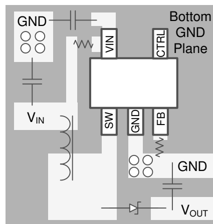
図 7-15. TPS61169 Board Layout
