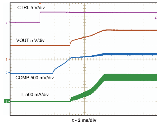
図 6. Start-Up
