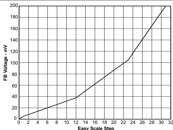
13. FB Voltage vs EasyScale Step
