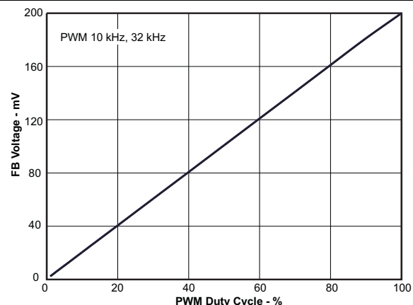
14. FB Voltage vs PWM Duty Cycle
