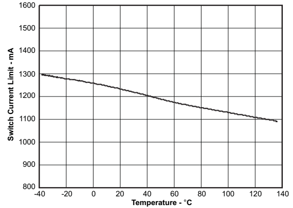
図 4. Switch Current Limit vs Temperature
