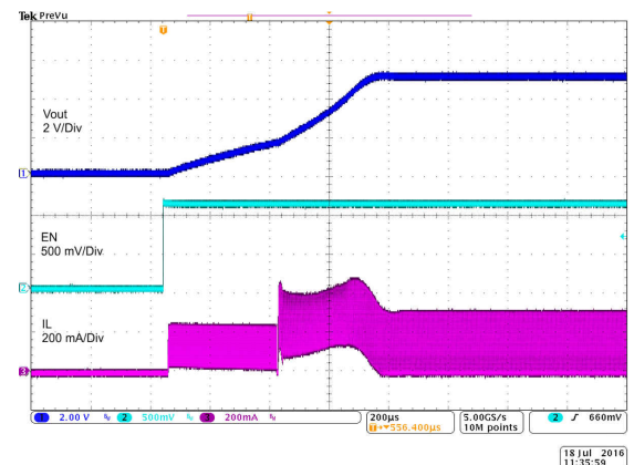
9-4. Startup by EN
