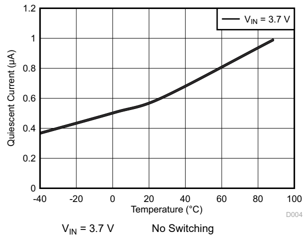
7-10. Quiescent Current into V_{OUT} vs Temperature
