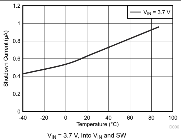
7-12. Shutdown Current vs Temperature
