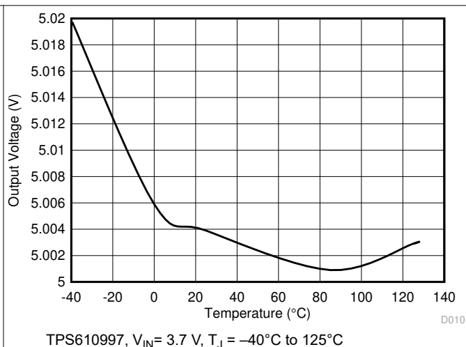
7-14. Output Voltage vs Temperature
