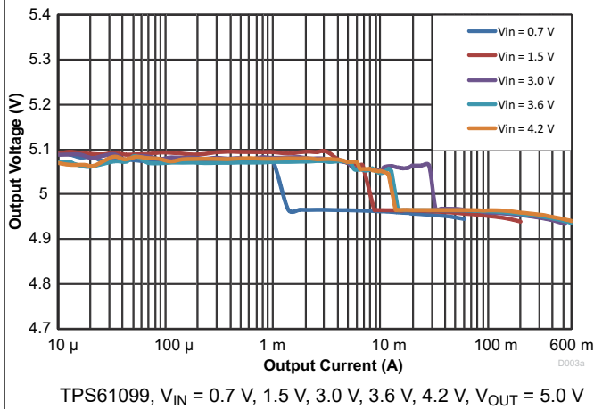
7-9. Load Regulation
