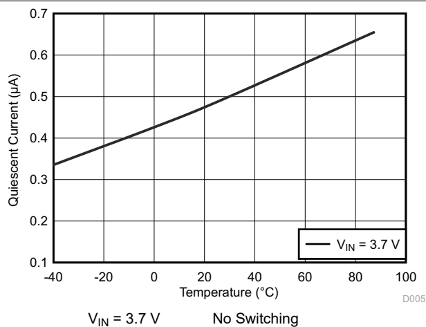
7-11. Quiescent Current into V_{IN} vs Temperature
