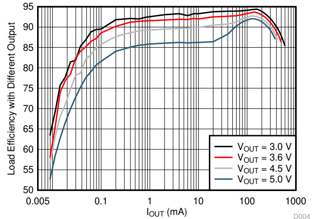
7-8. Load Efficiency with Different Outputs
