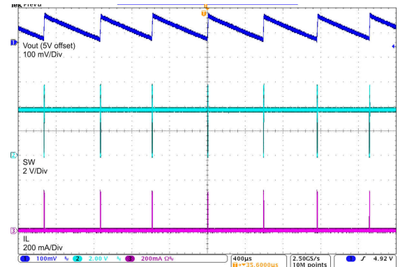
9-2. Switching Waveform at Light Load
