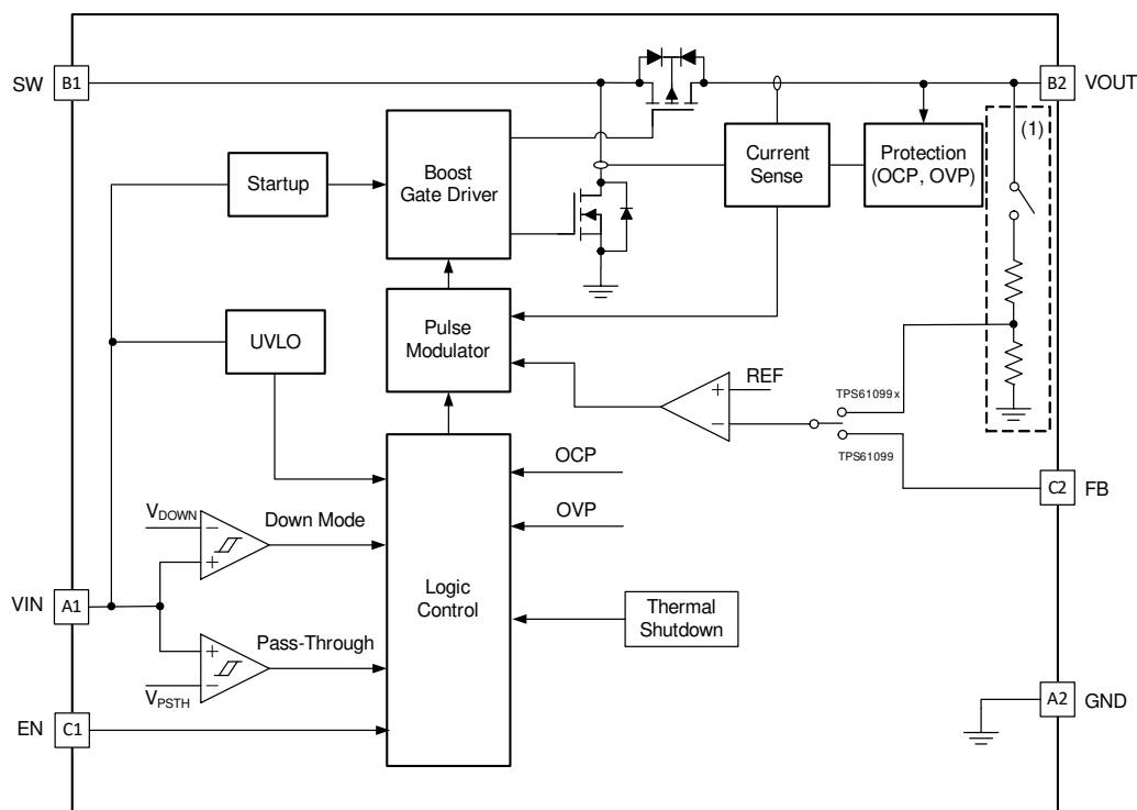
✎ 8-1. Functional Block Diagram
