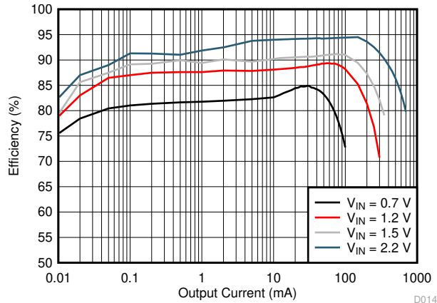
7-7. TPS610992 Load Efficiency with Different Inputs
