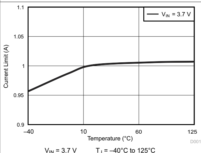
7-16. Current Limit vs Temperature
