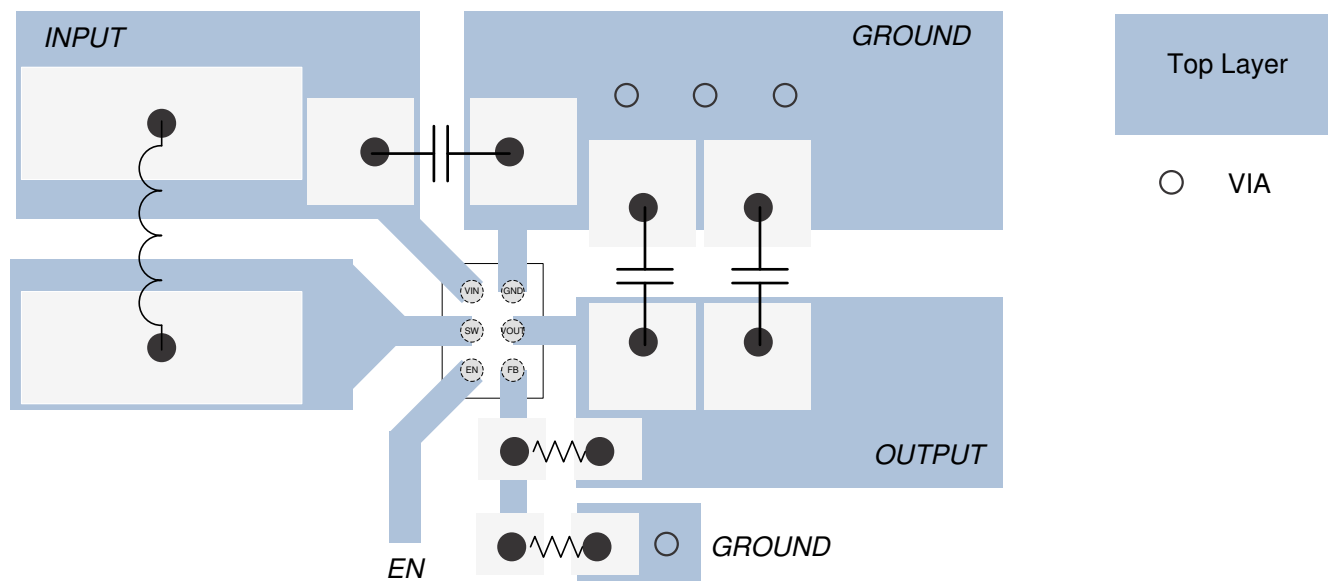
11-1. Layout -YFF
