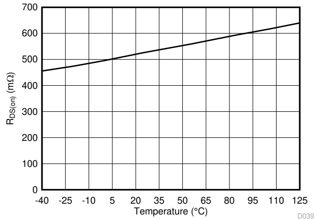
7-13. Rectifier on Resistance vs Temperature
