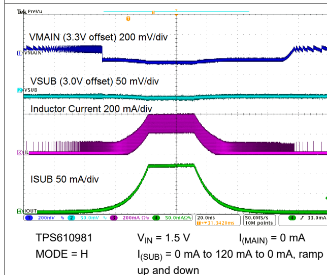
9-19. Load Regulation
