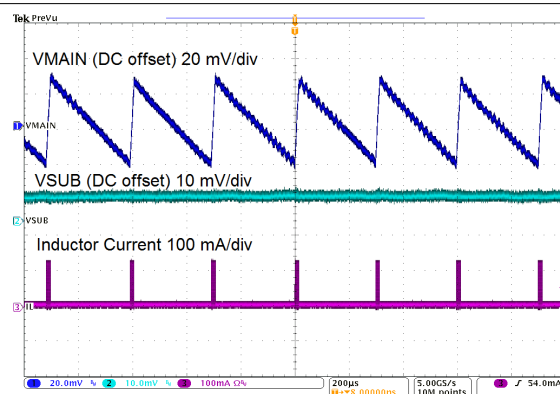
TPS610981 I_{(MAIN)} = 0 \text{ mA} I_{(SUB)} = 1 \text{ mA} MODE = H V_{IN} = 1.5 \text{ V}
