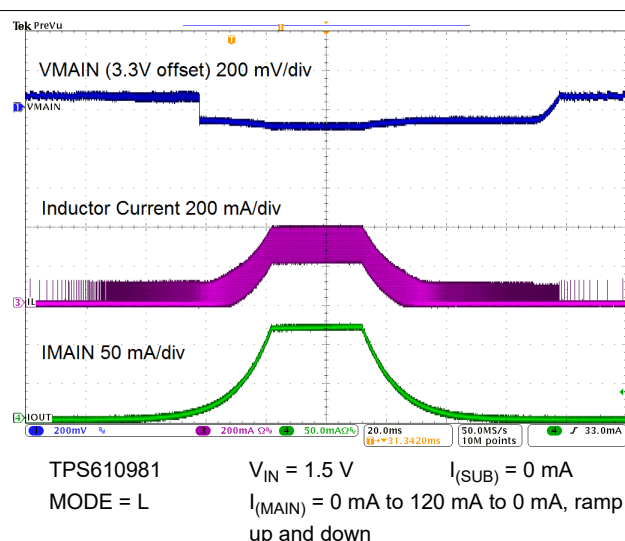
9-18. Load Regulation
