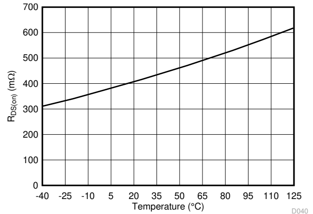
7-14. Low Side Switch On Resistance vs Temperature
