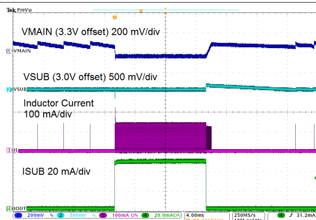
TPS610981 V_{IN} = 2.5 V I_{(MAIN)} = 0 mA MODE = H I_{(SUB)} = 0 mA to 50 mA, 5 \mu s rising/falling edge
