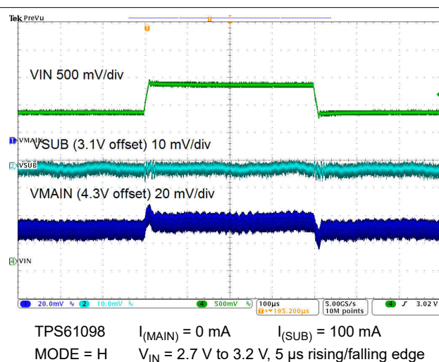
9-31. Line Transient Response
