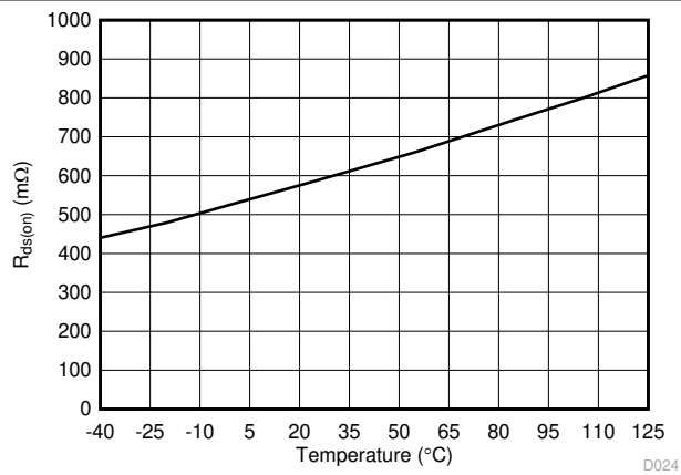
7-8. Low Side Switch On Resistance vs Temperature
