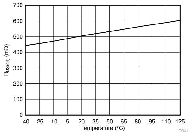
7-15. Rectifier on Resistance vs Temperature
