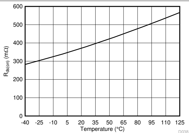
7-10. Low Side Switch On Resistance vs Temperature
