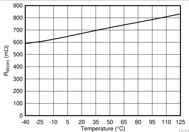
7-7. Rectifier On Resistance vs Temperature
