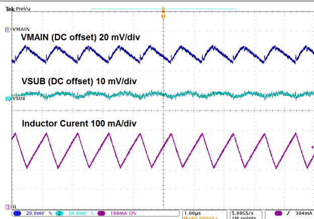
TPS610986 I_{(MAIN)} = 0 mA I_{(SUB)} = 100 mA MODE = H V_{IN} = 1.5 V
