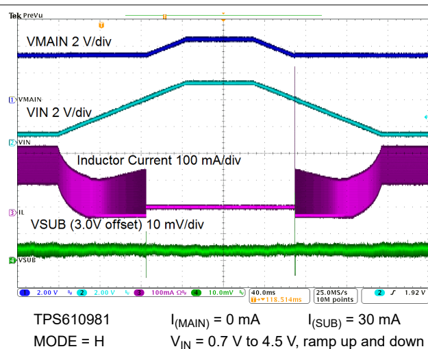
9-20. Line Regulation
