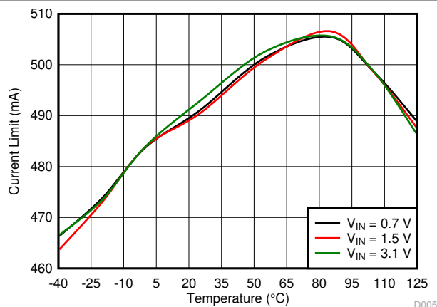
7-17. Current Limit vs Temperature
