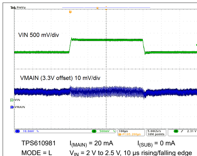
9-15. Line Transient Response
