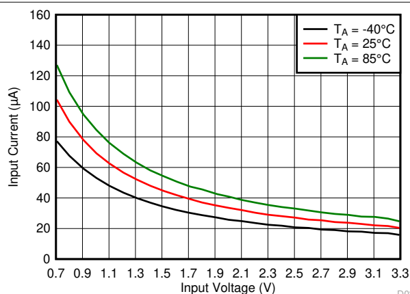
TPS610982 MODE = High No Load
