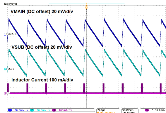
TPS610986 I_{(MAIN)} = 0 mA I_{(SUB)} = 1 mA MODE = H V_{IN} = 1.5 V
