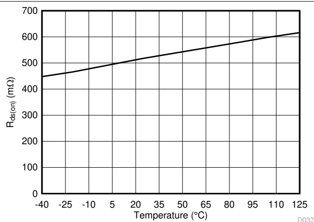
7-11. Rectifier On Resistance vs Temperature
