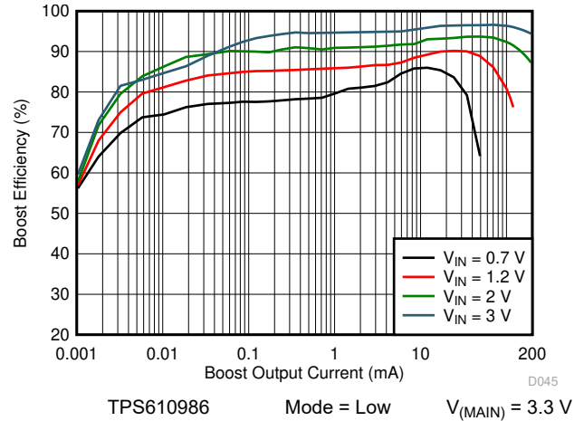
7-26. Boost Efficiency vs Output Current (Low Power Mode)
