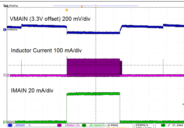
TPS610981 V_{IN} = 2.5 V I_{(SUB)} = 0 mA MODE = H I_{(MAIN)} = 0 mA to 50 mA, 5 \mu s rising/falling edge
