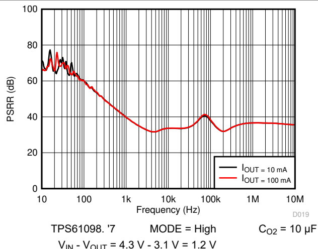
7-49. LDO PSRR vs Frequency
