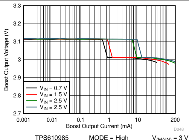
7-35. Boost Load Regulation (Active Mode)
