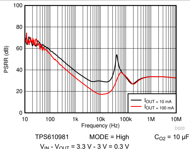
7-50. LDO PSRR vs Frequency
