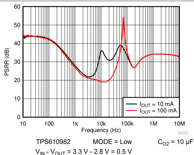
7-51. LDO PSRR vs Frequency (Low Power Mode)
