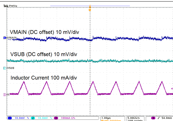
TPS610981 I_{(MAIN)} = 0 \text{ mA} I_{(SUB)} = 10 \text{ mA} MODE = H V_{IN} = 1.5 \text{ V}
