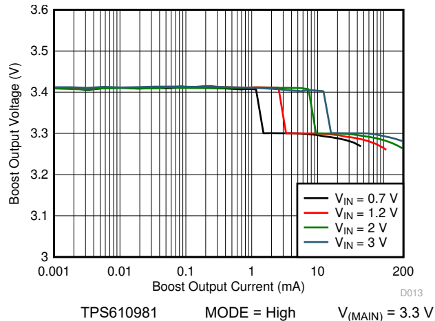
7-31. Boost Load Regulation (Active Mode)
