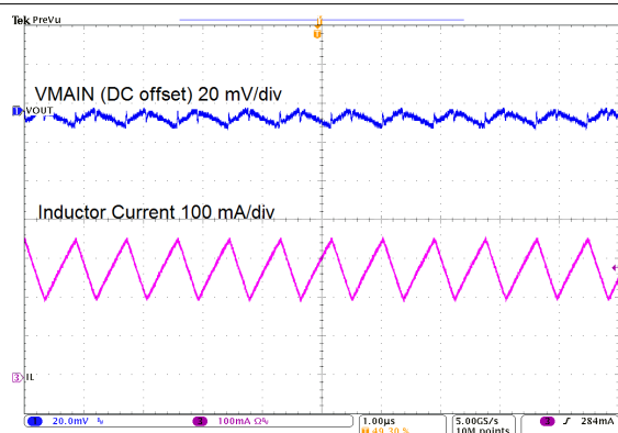
TPS610981 I_{(MAIN)} = 100 \text{ mA} I_{(SUB)} = 0 \text{ mA} MODE = L V_{IN} = 1.5 \text{ V}
