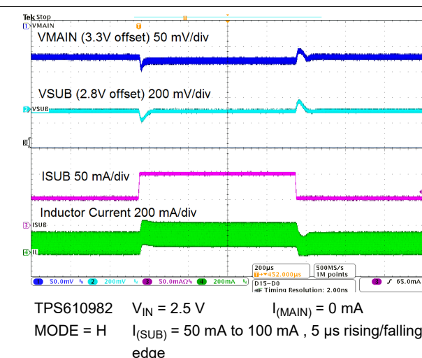
9-35. LDO Load Transient Response
