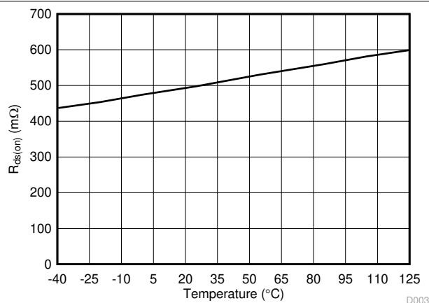
7-9. Rectifier On Resistance vs Temperature
