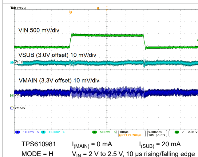
9-17. Line Transient Response
