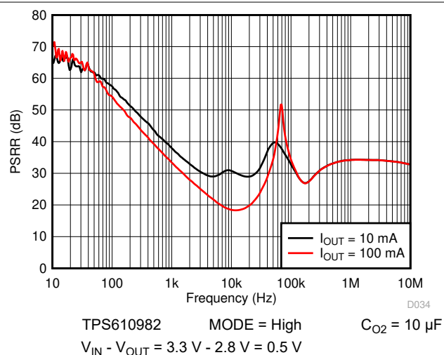
7-52. LDO PSRR vs Frequency (Active Mode)
