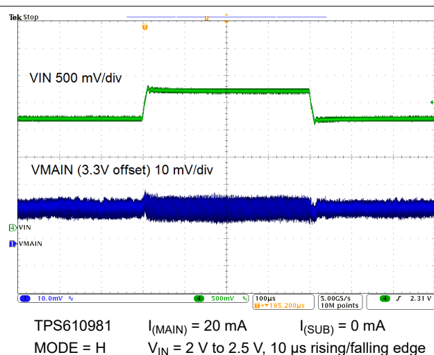
9-16. Line Transient Response
