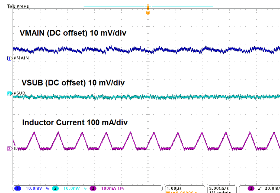
TPS610986 I_{(MAIN)} = 0 mA I_{(SUB)} = 10 mA MODE = H V_{IN} = 1.5 V
