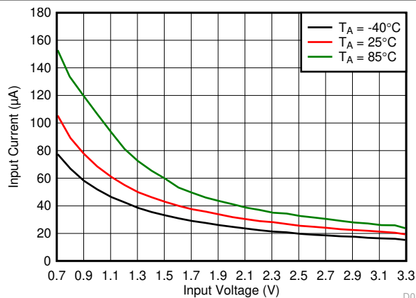
TPS610981 MODE = High No Load
