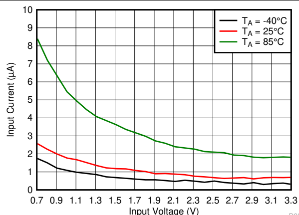
TPS610986 MODE = Low V_{(\text{MAIN})} = 3.3\text{ V}
