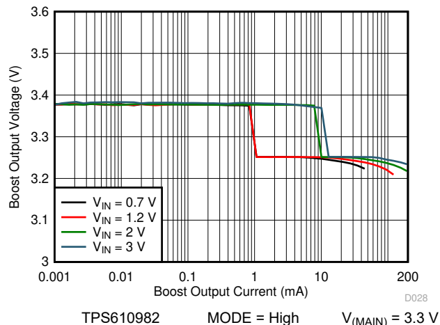
7-33. Boost Load Regulation (Active Mode)
