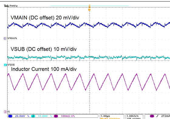
TPS610981 I_{(MAIN)} = 0 \text{ mA} I_{(SUB)} = 100 \text{ mA} MODE = H V_{IN} = 1.5 \text{ V}
