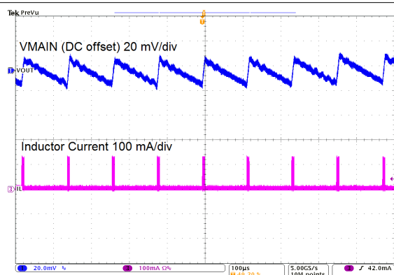
TPS610981 I_{(MAIN)} = 1 \text{ mA} I_{(SUB)} = 0 \text{ mA} MODE = L V_{IN} = 1.5 \text{ V}
