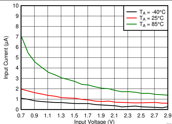
TPS610985 MODE = Low V_{(\text{MAIN})} = 3\text{ V}
