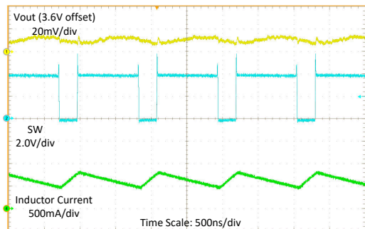
8-2. Switching Waveform at Heavy Load
