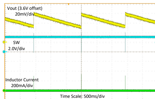
8-3. Switching Waveform at Medium Load
