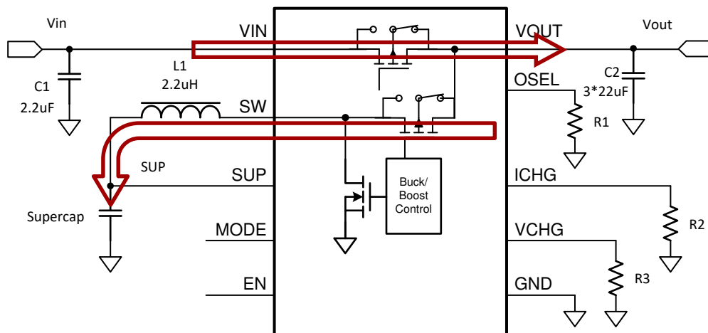
7-3. Typical Buck_on State Circuit
