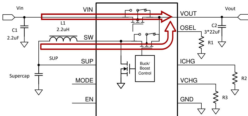
7-4. Typical Supplement State Circuit
