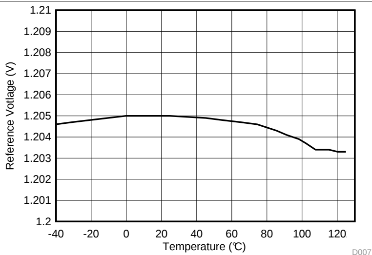
FIG 11. Reference Voltage vs Temperature
