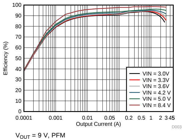
FIG 3. Efficiency vs Output Current
