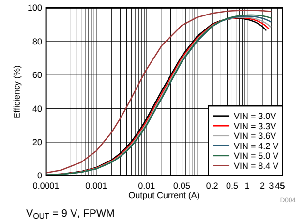
FIG 4. Efficiency vs Output Current
