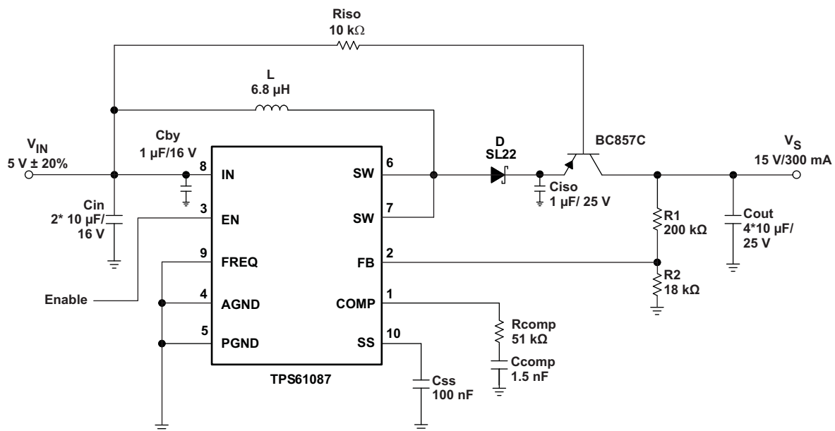
Figure 17. Typical Application With External Load Disconnect Switch
