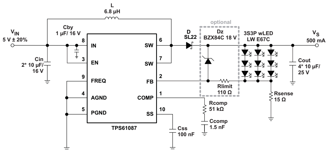
Figure 20. Simple Application (5 V Input Voltage) ( f_s = 650\text{ kHz} ) for wLED Supply (3S3P) (With Optional Clamping Zener Diode)
