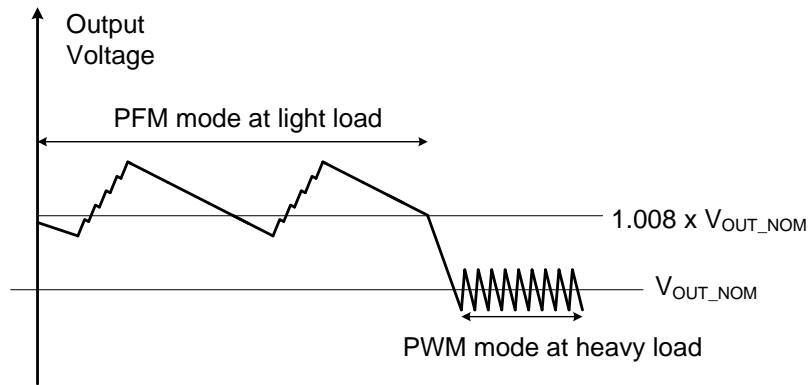
FIG 10. Output Voltage in PWM Mode and PFM Mode
