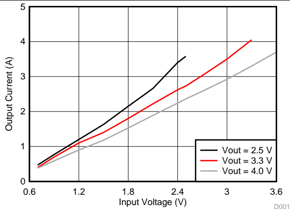
V_{IN} = 0.7\text{ V} to 3.6\text{ V} , V_{OUT} = 2.5\text{ V} , 3.3\text{ V} , 4.0\text{ V}
