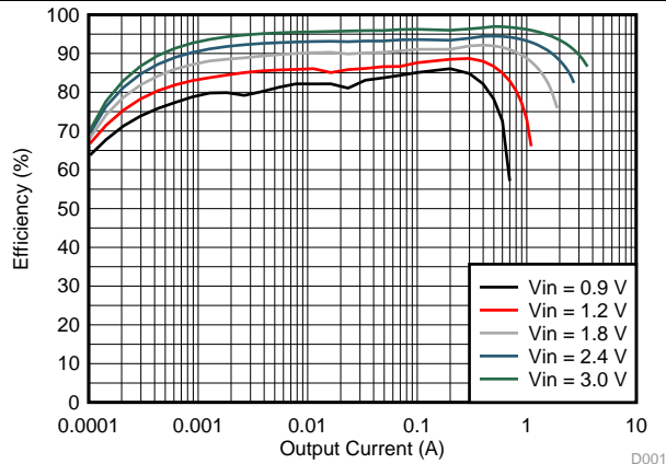
V_{IN} = 0.9\text{ V} , 1.2\text{ V} , 1.8\text{ V} , 2.4\text{ V} , 3.0\text{ V} , and V_{OUT} = 3.3\text{ V}
