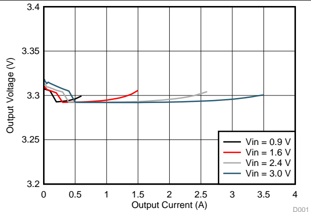
V_{IN} = 0.9\text{ V} , 1.6\text{ V} , 2.4\text{ V} , 3.0\text{ V} , and V_{OUT} = 3.3\text{ V}
