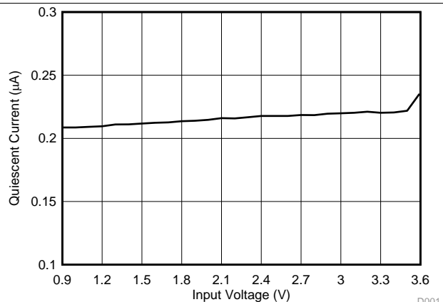
V_{IN} = 0.9\text{ V} to 3.6\text{ V} , V_{OUT} = 4.0\text{ V} , No switching
