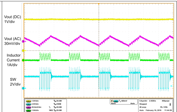
13. Switching Waveform at Light Load
