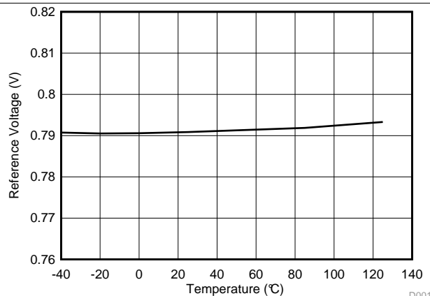
V_{IN} = 2.4\text{ V} , V_{OUT} = 3.3\text{ V} , T = -40^\circ\text{C} to 125^\circ\text{C}
