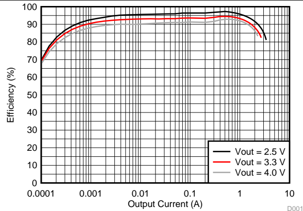
V_{IN} = 2.4\text{ V} , and V_{OUT} = 2.5\text{ V} , 3.3\text{ V} , 4.0\text{ V}
