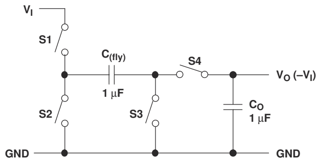
FIG 8-1. Operating Principle
