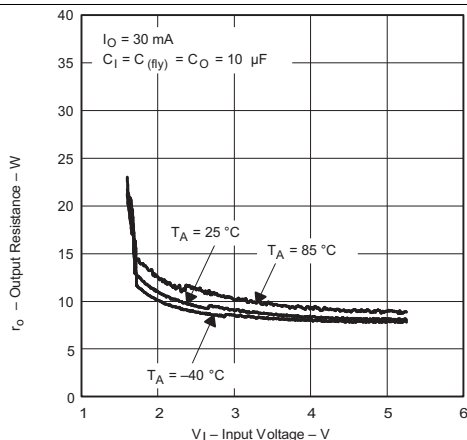
Figure 8. TPS60401-Q1 Output Resistance vs Input Voltage
