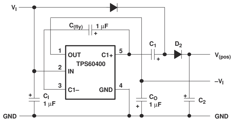
FIG 9-7. TPS60400 as Doubler/Inverter
