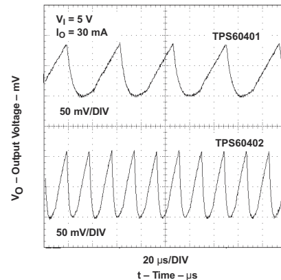
9-3. Output Voltage vs Time for TPS60401 and TPS60402
