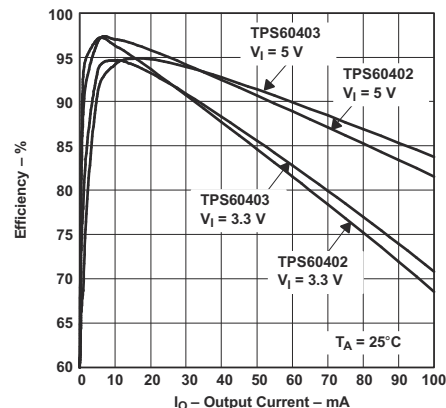
7-2. Efficiency vs Output Current
