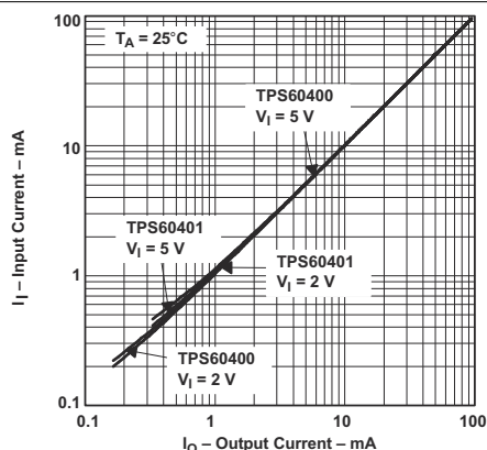
7-3. Input Current vs Output Current
