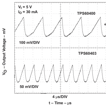
9-2. Output Voltage vs Time for TPS60400 and TPS60401
