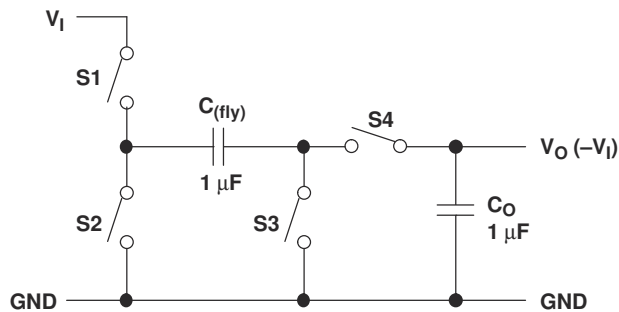
FIG 8-1. Operating Principle
