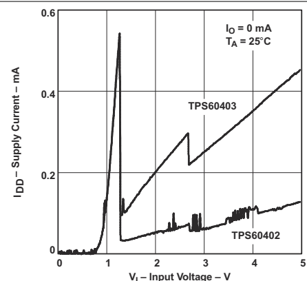
7-6. Supply Current vs Input Voltage
