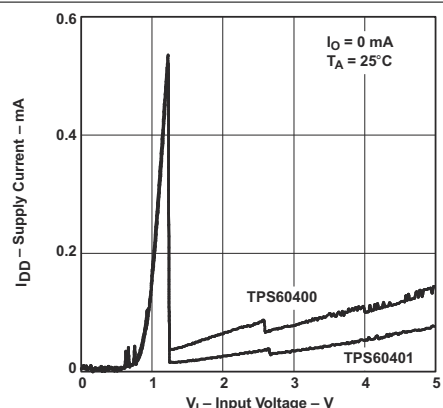
7-5. Supply Current vs Input Voltage
