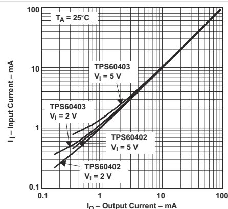
7-4. Input Current vs Output Current
