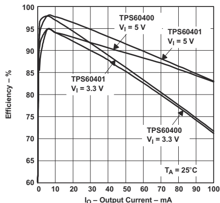
7-1. Efficiency vs Output Current
