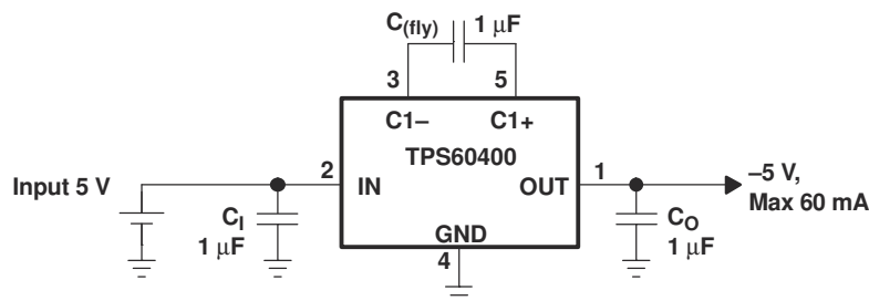
FIG 9-1. Typical Operating Circuit
