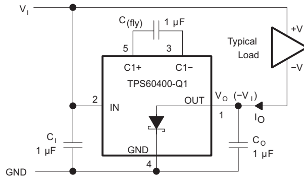
Figure 21. Typical Load
