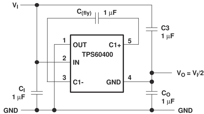
FIG 9-6. TPS60400 as a High-Efficiency Rail Splitter
