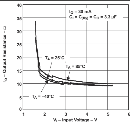
☒ 7-9. Output Resistance vs Input Voltage
