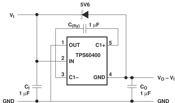
Figure 9-14. Step-Down Charge Pump Connection for Higher Input Voltages
