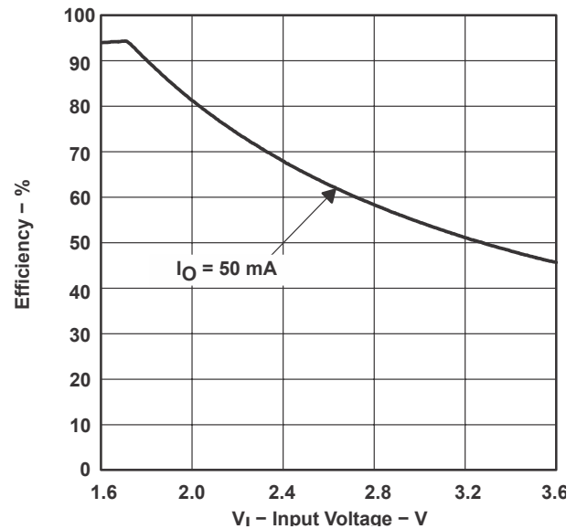
図 7-2. Efficiency vs Input Voltage
