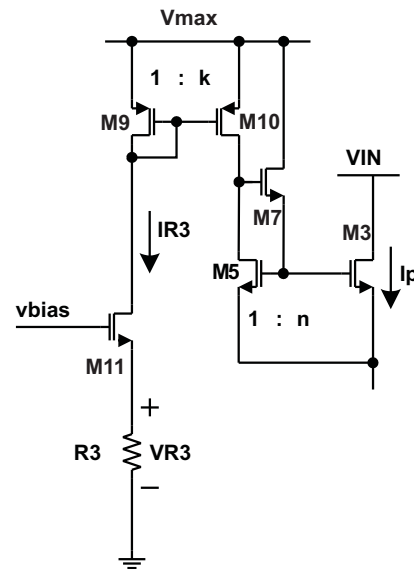
Figure 8. Current Limit
