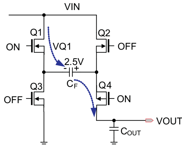
Figure 4. Discharging Mode
