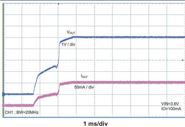
Figure 22. Power On V IN = 3.6 V, I o = 100 mA
