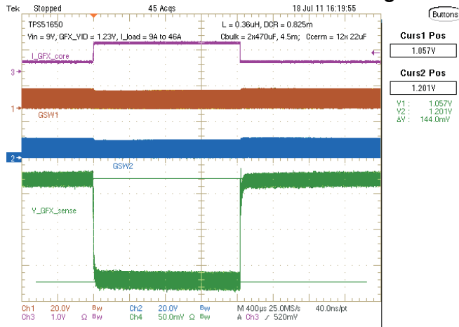
Figure 25. Load Transient, V_{IN} = 9\text{ V} , Load Step = 37 A
