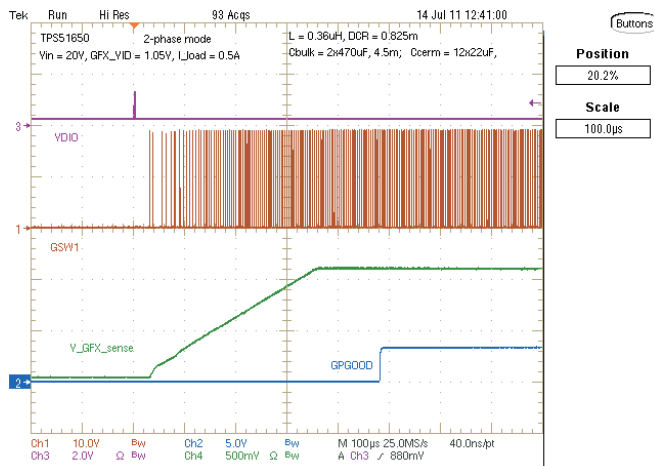
Figure 29. Start-Up and PGOOD
