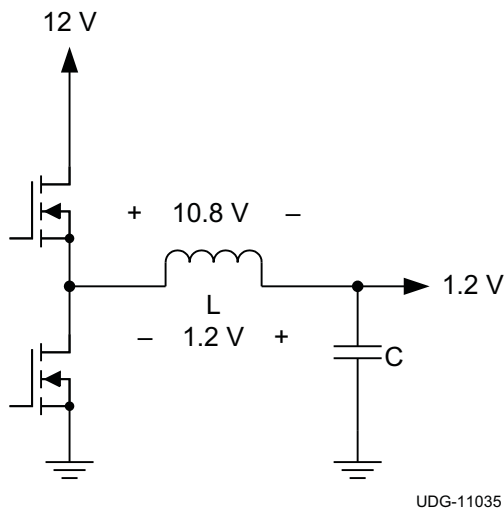
Figure 45. Synchronous Converter
