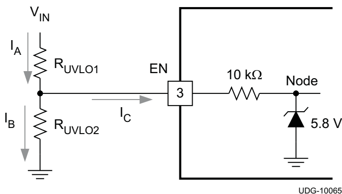
Figure 29. Node Voltage
