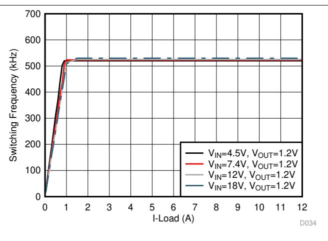
図 22. Switching Frequency vs Output Load
