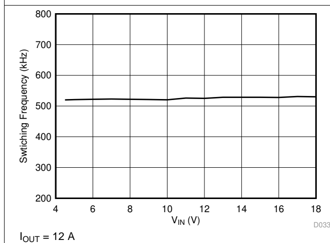
図 21. Switching Frequency vs Input Voltage
