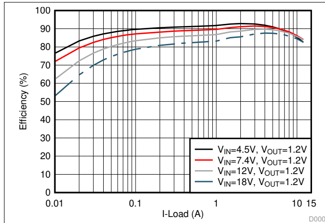
図 19. Efficiency Curve
