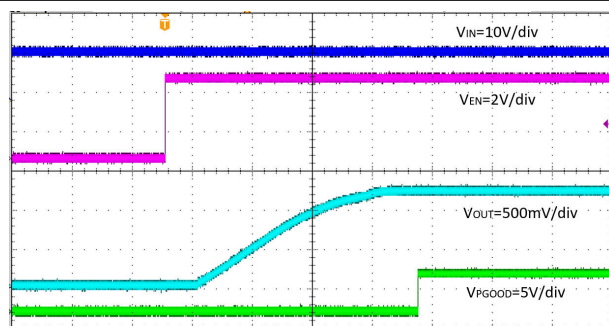
8-6. Start-Up Relative to EN Rising, Time = 2 ms/div
