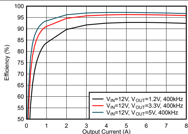
Figure 6-18. Efficiency, Mode = FCCM, f_{sw} = 400\text{ kHz}
