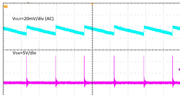
8-4. Output Voltage Ripple, I_{OUT} = 10\text{ mA} , Time = 80 \mu\text{s/div}
