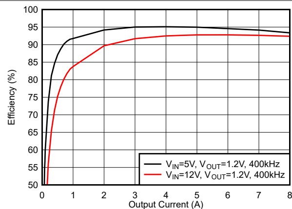
Figure 6-12. Efficiency, Mode = FCCM, f_{SW} = 400\text{ kHz}
