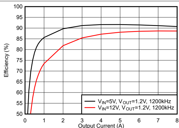
Figure 6-16. Efficiency, Mode = FCCM, f_{sw} = 1200\text{ kHz}
