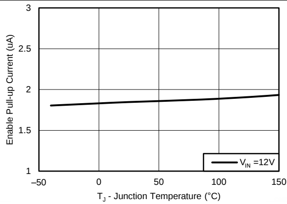
図 7. Enable Pull-Up Current, V_{EN} = 1.0V
