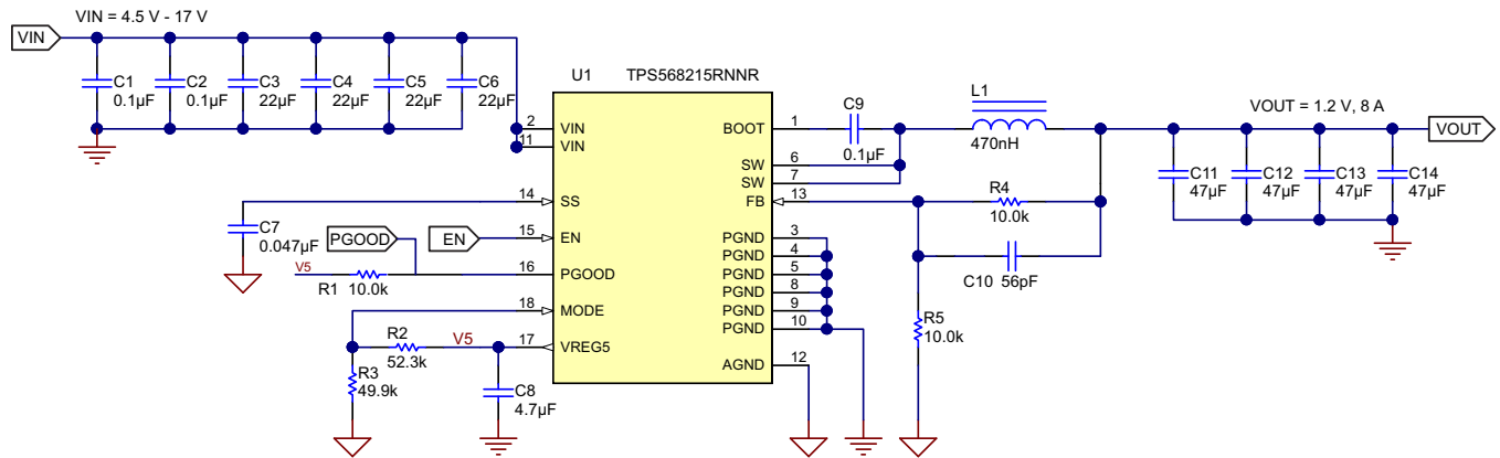
22. Application Schematic
