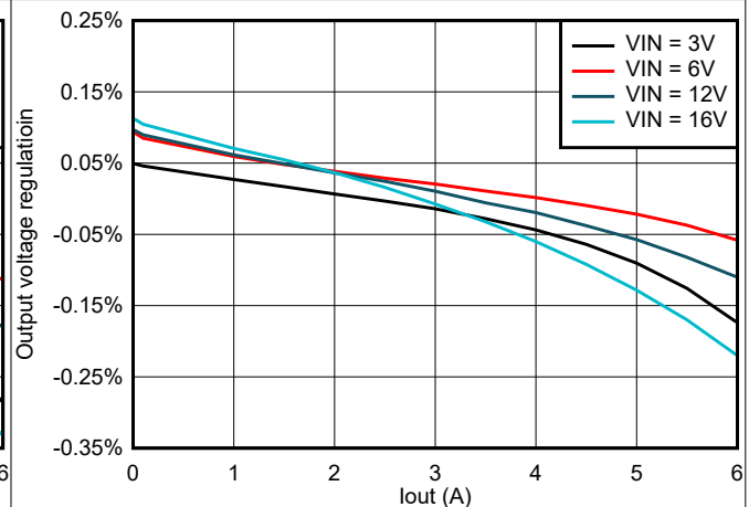
8-5. TPS566247 Load Regulation vs Loading
