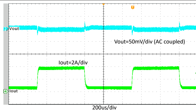
8-17. TPS564255 Transient Response with 0.4 A to 3.6 A
