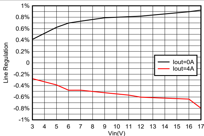
8-8. TPS564252 Line Regulation vs V_{IN}
