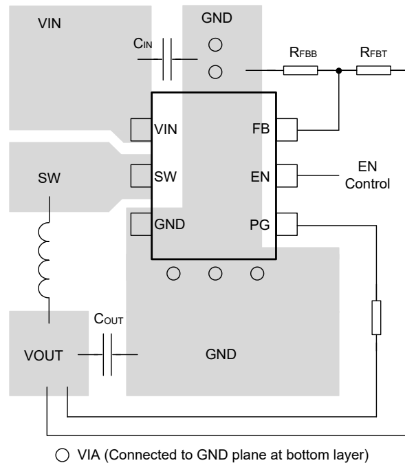
8-26. Suggested Layout
