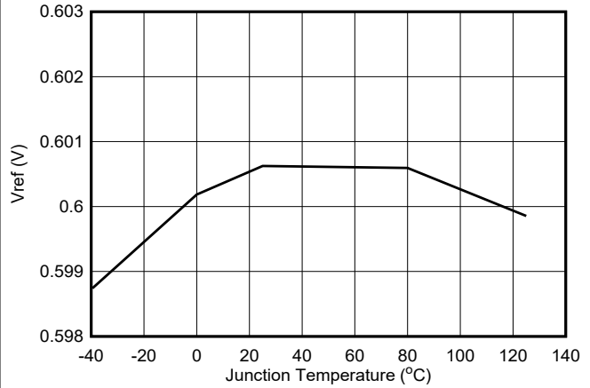
Figure 6-8. V_{REF} Voltage
