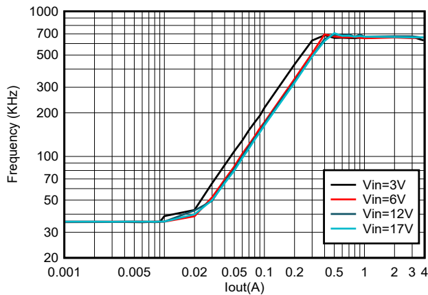
8-4. TPS564255 Frequency vs Loading
