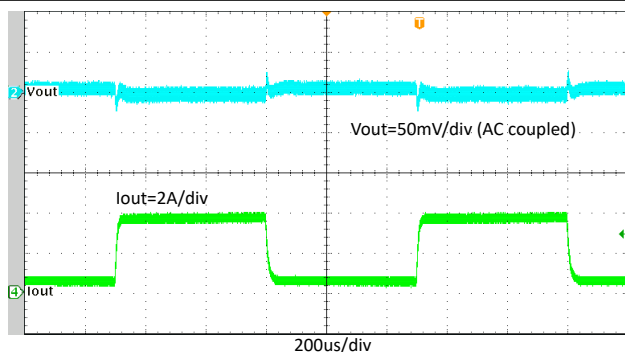
8-16. TPS564257 Transient Response with 0.4 A to 3.6 A
