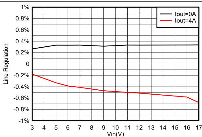
8-10. TPS564255 Line Regulation vs V_{IN}
