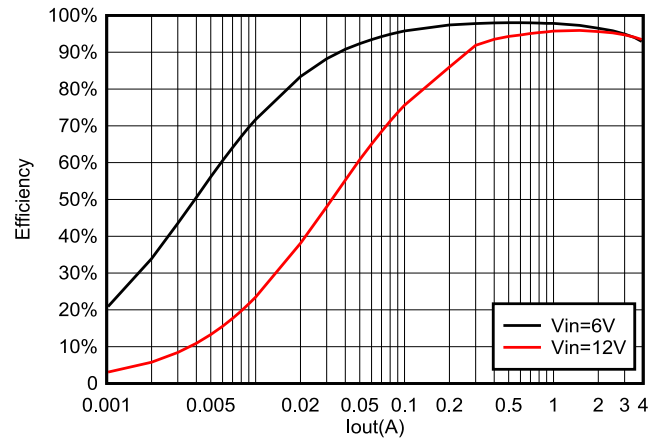
6-20. TPS564257 Efficiency at 5 V_{OUT} with a 4.7- \mu\text{H} Inductor
