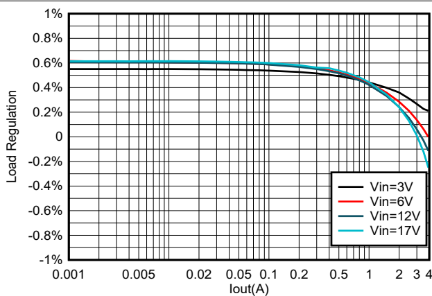
8-6. TPS564257 Load Regulation vs Loading
