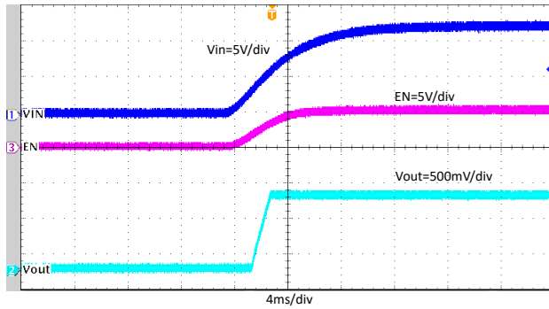
8-20. Start-Up with V_{IN} Rising, I_{OUT} = 4\text{ A}
