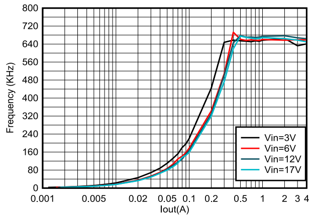
8-2. TPS564252 Frequency vs Loading
