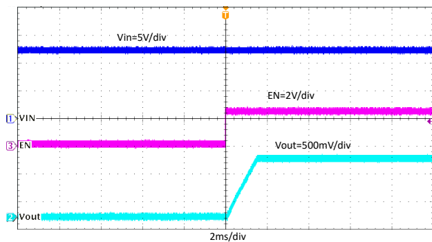
8-18. Start-Up Through EN, I_{OUT} = 4 A
