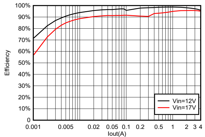
6-22. TPS564252 Efficiency at 10 V_{OUT} with a 6.8- \mu\text{H} Inductor
