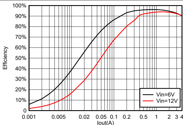
FIG 6-17. TPS564257 Efficiency at 3.3 V_{OUT} with a 3.3- \mu\text{H} Inductor
