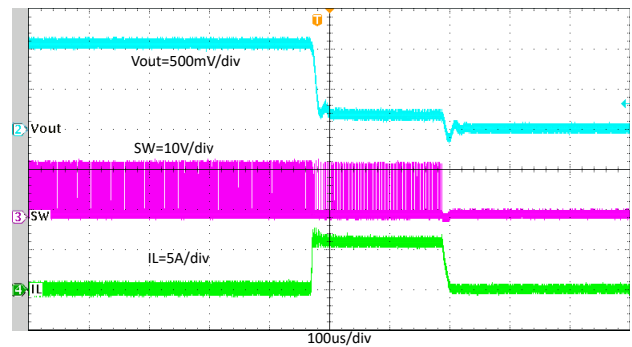
8-23. TPS564257 Normal Operation to Output Hard Short
