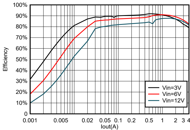
FIG 6-15. TPS564255 Efficiency at 1.05 V_{OUT} with a 1.5- \mu\text{H} Inductor
