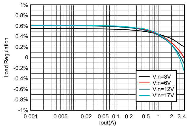
8-5. TPS564252 Load Regulation vs Loading
