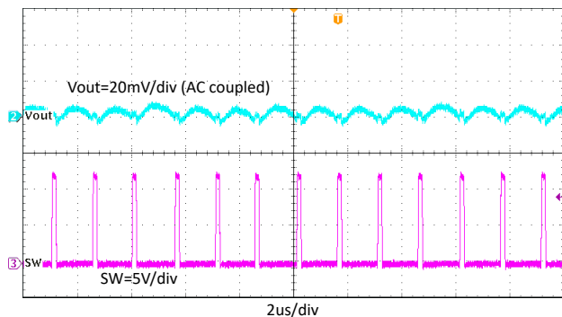
8-14. Output Voltage Ripple with 4-A Loading
