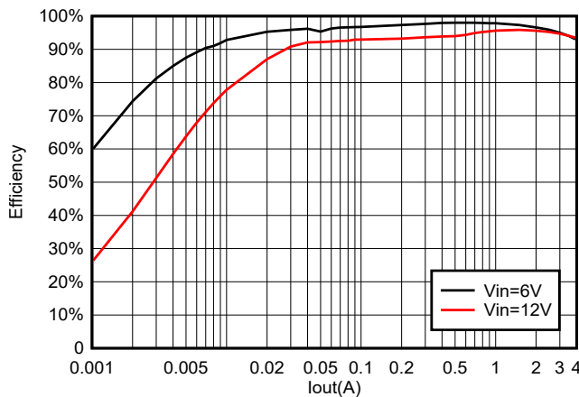
6-21. TPS564255 Efficiency at 5 V_{OUT} with a 4.7- \mu\text{H} Inductor
