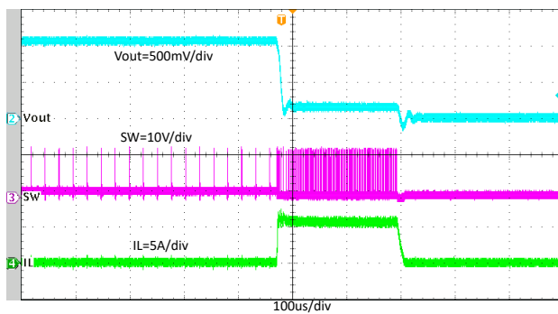
8-24. TPS564255 Normal Operation to Output Hard Short
