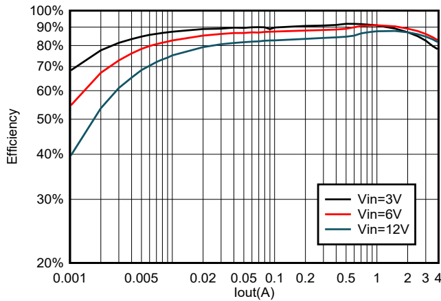
FIG 6-13. TPS564252 Efficiency at 1.05 V_{OUT} with a 1.5- \mu\text{H} Inductor
