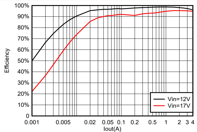
6-24. TPS564255 Efficiency at 10 V_{OUT} with a 6.8- \mu\text{H} Inductor
