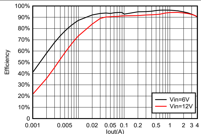
FIG 6-18. TPS564255 Efficiency at 3.3 V_{OUT} with a 3.3- \mu\text{H} Inductor
