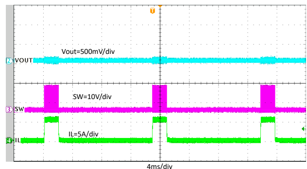
8-25. Output Hard Short Hiccup
