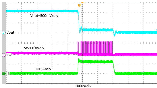
8-22. TPS564252 Normal Operation to Output Hard Short
