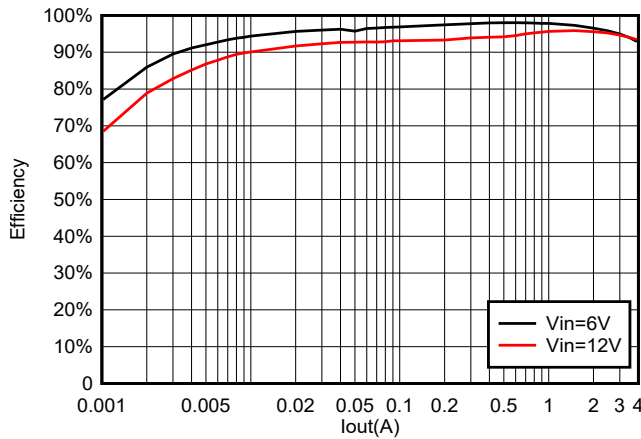
6-19. TPS564252 Efficiency at 5 V_{OUT} with a 4.7- \mu\text{H} Inductor
