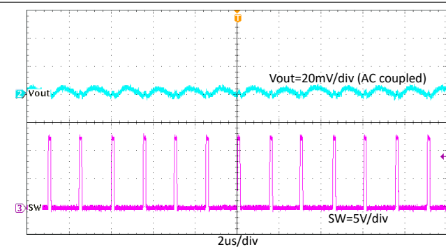
8-12. TPS564257 Output Voltage Ripple with 0.01-A Loading
