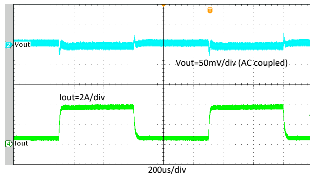
8-15. TPS564252 Transient Response with 0.4 A to 3.6 A
