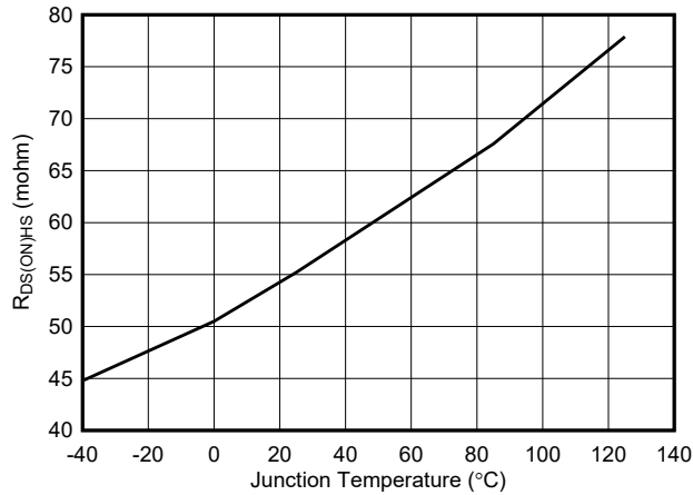
Figure 6-7. High-Side R_{DS(on)}
