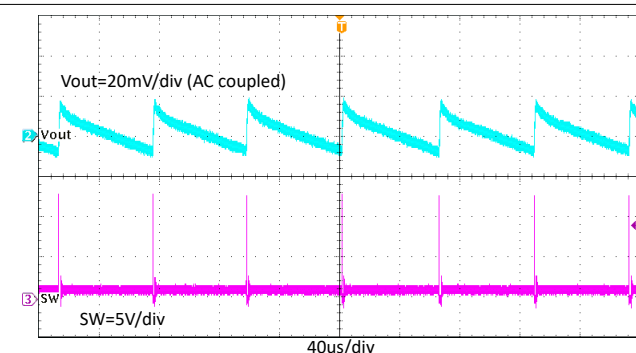
8-11. TPS564252 Output Voltage Ripple with 0.01-A Loading
