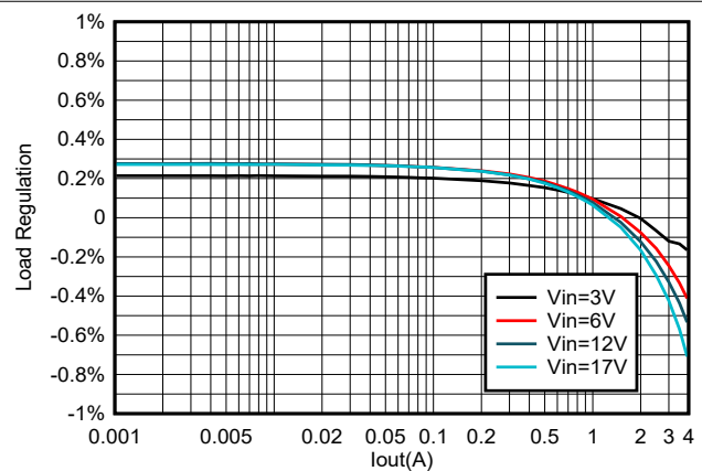
8-7. TPS564255 Load Regulation vs Loading
