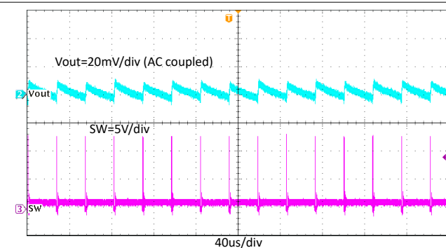
8-13. TPS564255 Output Voltage Ripple with 0.01-A Loading
