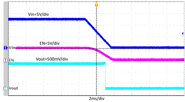
8-21. Shutdown with V_{IN} Falling, I_{OUT} = 4\text{ A}
