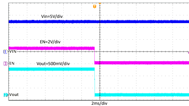
8-19. Shutdown Through EN, I_{OUT} = 4 A
