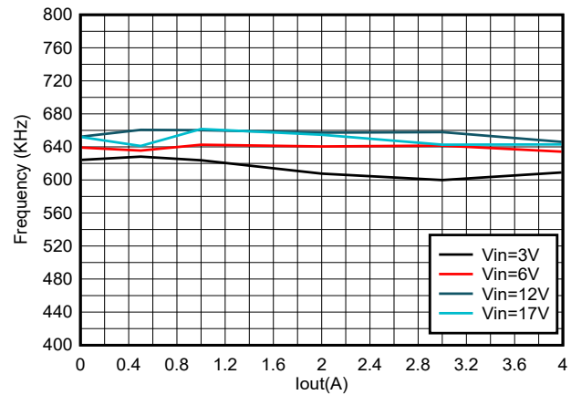
8-3. TPS564257 Frequency vs Loading
