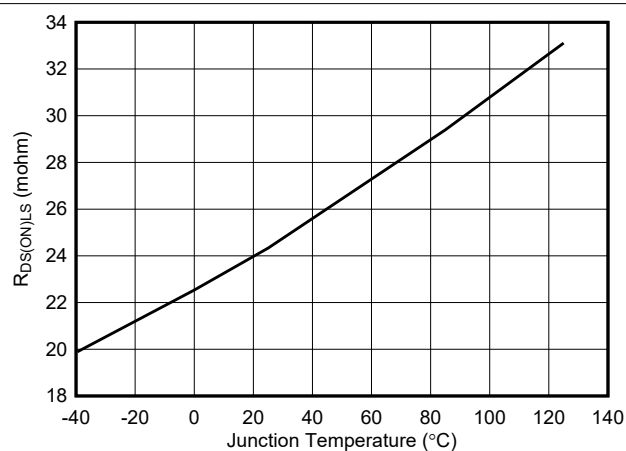
Figure 6-6. Low-Side R_{DS(ON)}
