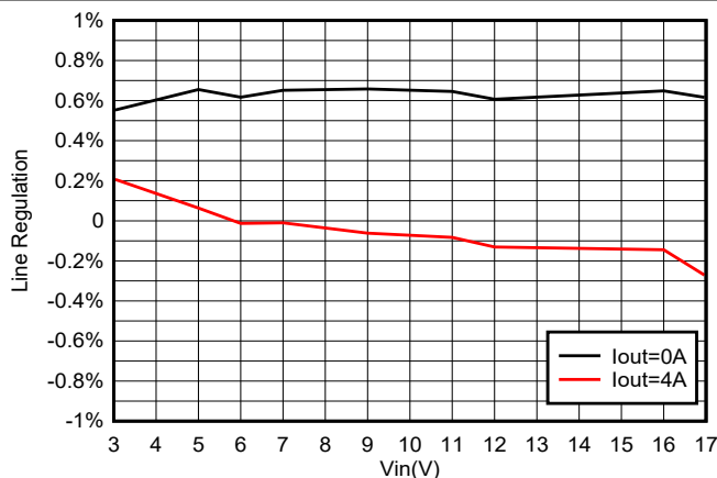
8-9. TPS564257 Line Regulation vs V_{IN}
