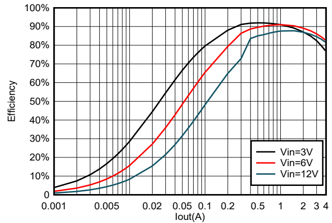
FIG 6-14. TPS564257 Efficiency at 1.05 V_{OUT} with a 1.5- \mu\text{H} Inductor
