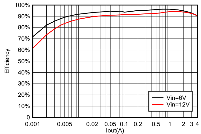
FIG 6-16. TPS564252 Efficiency at 3.3 V_{OUT} with a 3.3- \mu\text{H} Inductor
