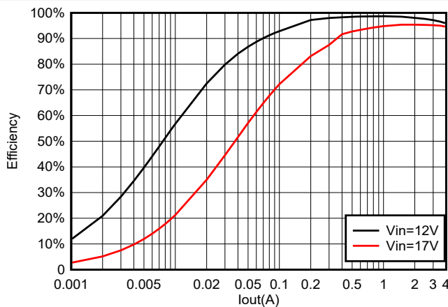
6-23. TPS564257 Efficiency at 10 V_{OUT} with a 6.8- \mu\text{H} Inductor
