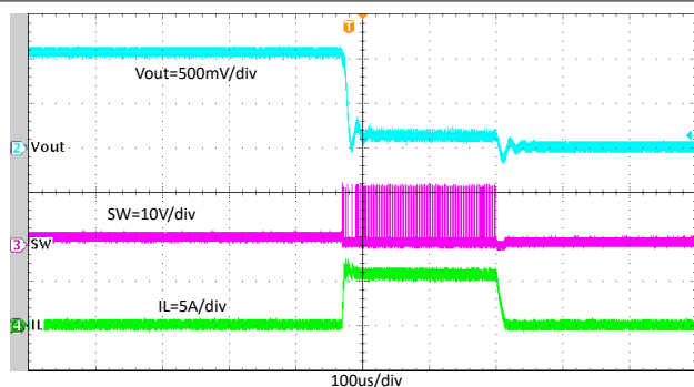
8-22. TPS564252 Normal Operation to Output Hard Short
