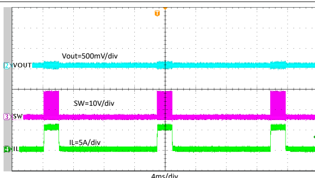
8-25. Output Hard Short Hiccup
