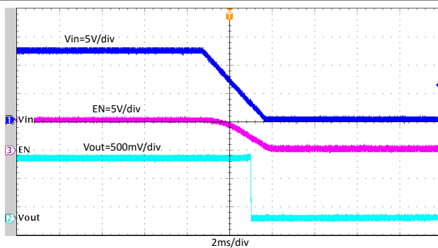
8-21. Shutdown with V_{IN} Falling, I_{OUT} = 4\text{ A}
