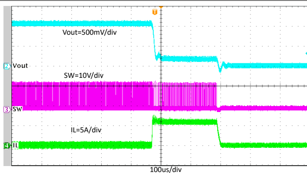
8-23. TPS564257 Normal Operation to Output Hard Short
