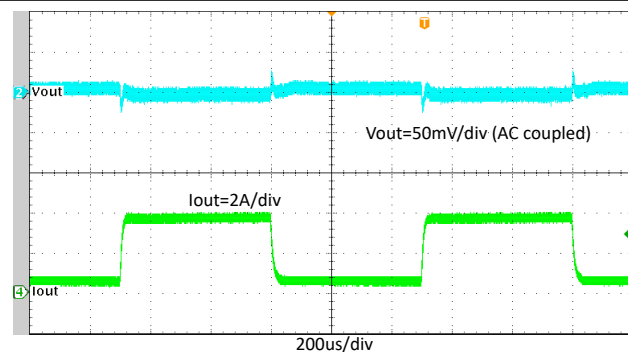
8-17. TPS564255 Transient Response with 0.4 A to 3.6 A
