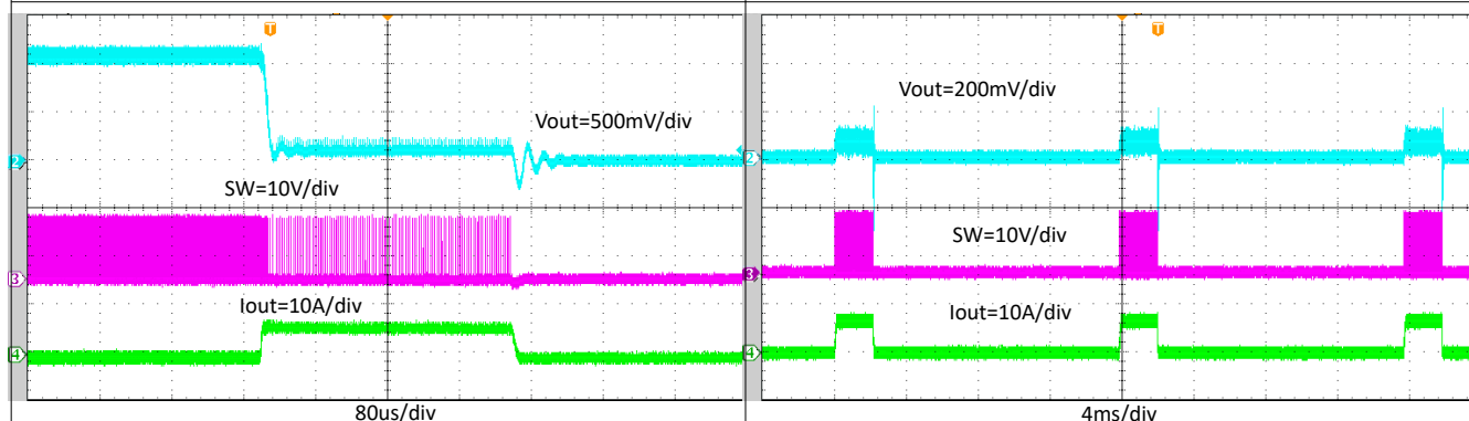
8-20. TPS564247 Normal Operation to Output Hard Short
