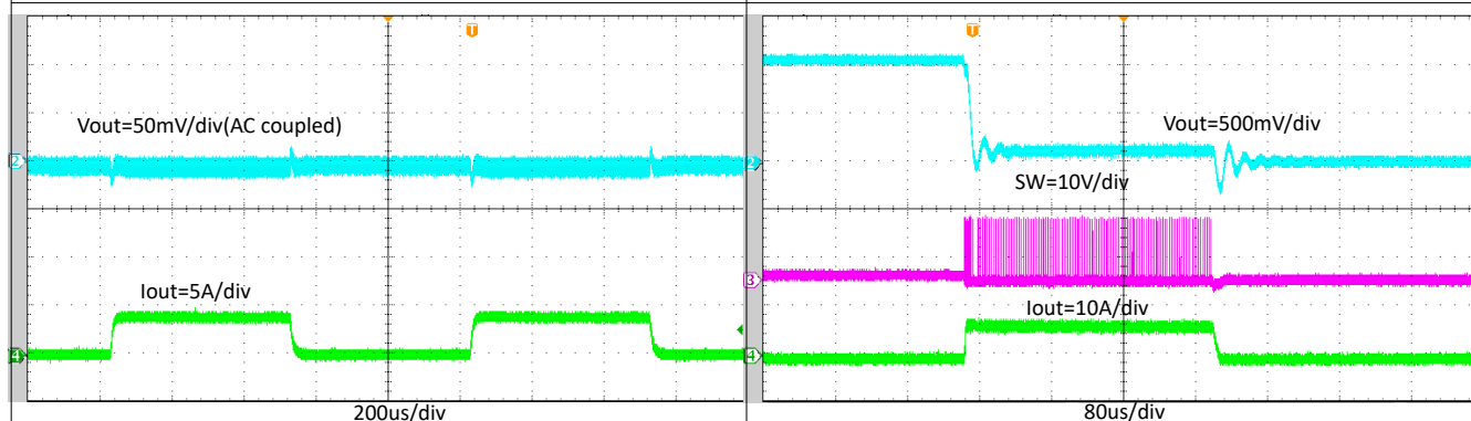
8-18. TPS564247 Transient Response with 0.1 A to 4 A by 2.5-A/μs Load Step
