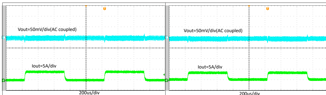
8-16. TPS564242 Transient Response with 0.1 A to 4 A by 2.5-A/μs Load Step
