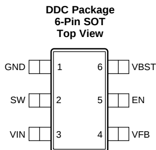
Pin Functions
