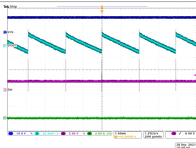
8-6. Steady State Waveforms, I_{OUT} = 0\text{ A}
