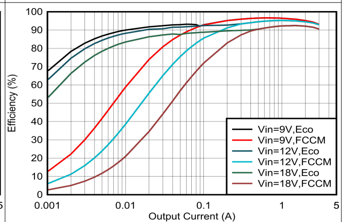
FIG 6-16. V_{OUT} = 7\text{-V} Efficiency, L = 3.3\text{ }\mu\text{H}
