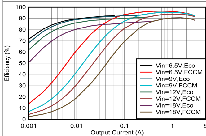
FIG 6-15. V_{OUT} = 5\text{-V} Efficiency, L = 3.3\text{ }\mu\text{H}
