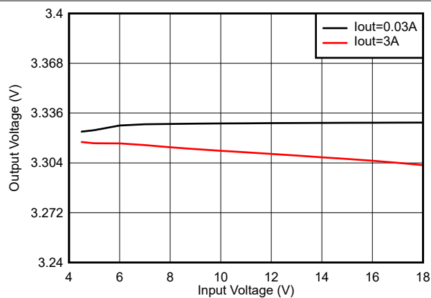
8-4. Line Regulation
