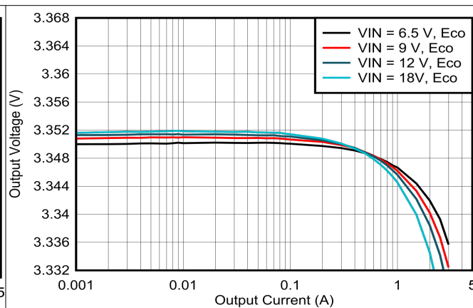
8-3. Load Regulation
