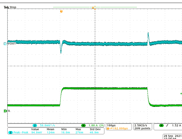
8-11. Transient Response 0.5 to 2 A with Slew Rate of 2.5\text{ A}/\mu\text{s}
