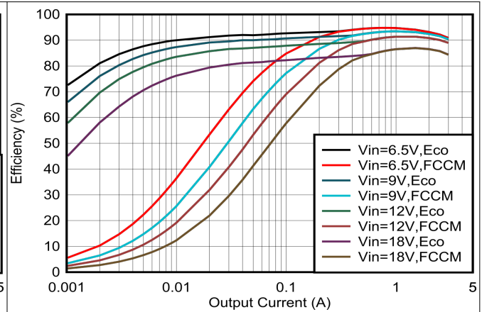
FIG 6-14. V_{OUT} = 3.3\text{-V} Efficiency, L = 2.2\text{ }\mu\text{H}
