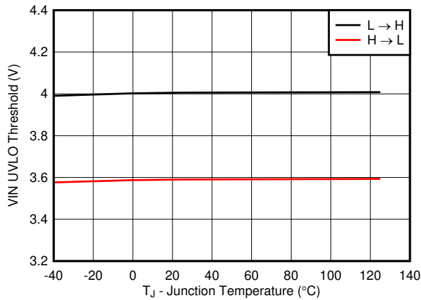
6-7. VIN UVLO Threshold vs Junction Temperature
