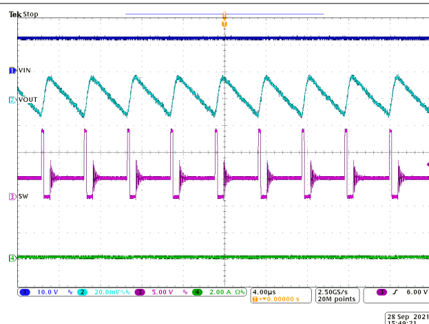
8-7. Steady State Waveforms, I_{OUT} = 0.1\text{ A}
