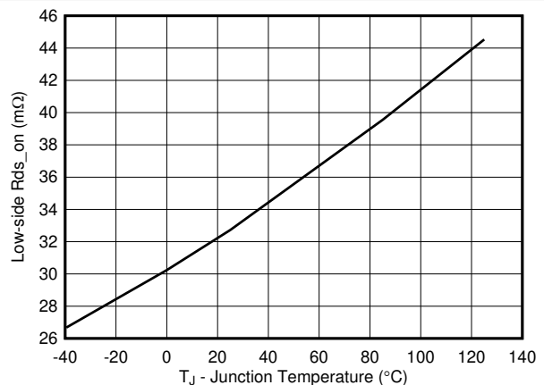
FIG 6-6. Low-Side MOSFET On-Resistance vs Junction Temperature
