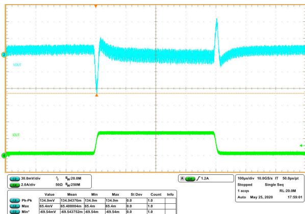
图 8-14. Transient Response 0.3 to 2.7 A with Slew Rate of 0.25 A/μs
