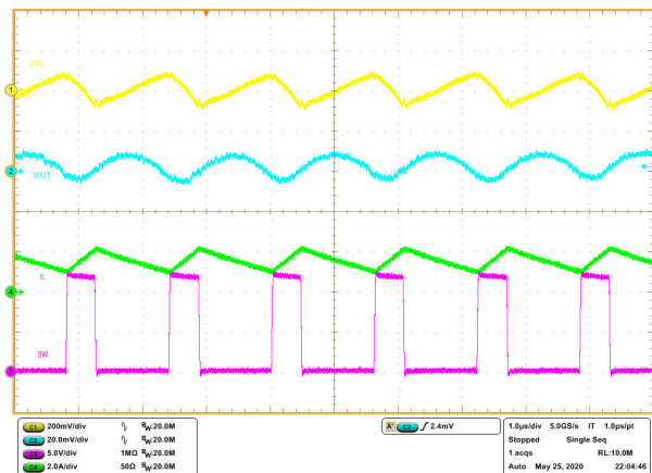
图 8-8. Steady State Waveforms, I_{OUT} = 1.5\text{ A}
