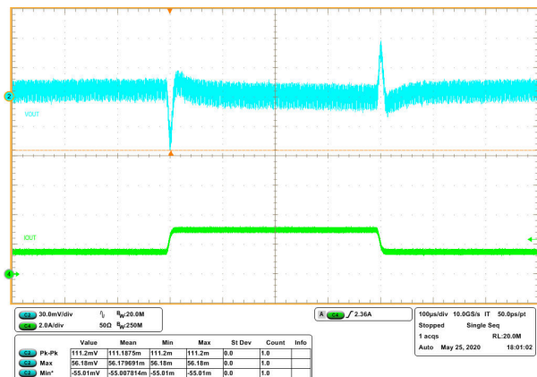
图 8-15. Transient Response 1.5 to 3 A with Slew Rate of 0.25 A/μs
