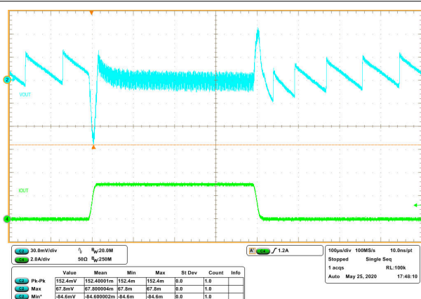
图 8-10. Transient Response 0 to 3 A with Slew Rate of 0.25\text{ A}/\mu\text{s} (Eco-Mode)
