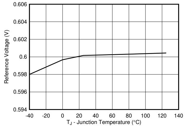
FIG 6-4. Reference Voltage vs Junction Temperature
