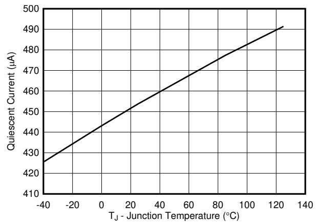
FIG 6-2. Quiescent Current (FCCM) vs Junction Temperature
