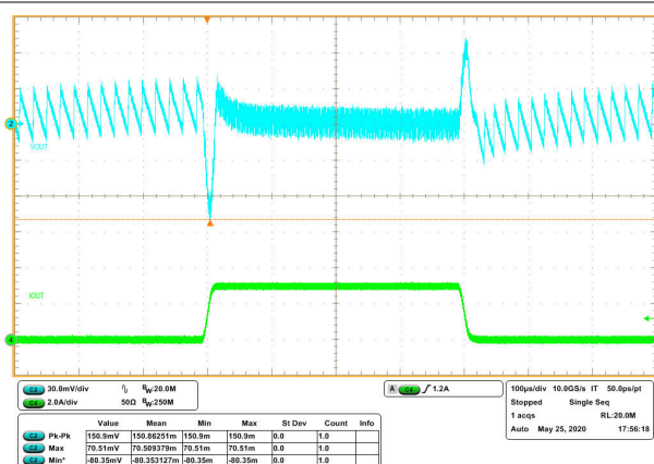
图 8-12. Transient Response 0.03 to 3 A with Slew Rate of 0.25\text{ A}/\mu\text{s} (Eco-Mode)
