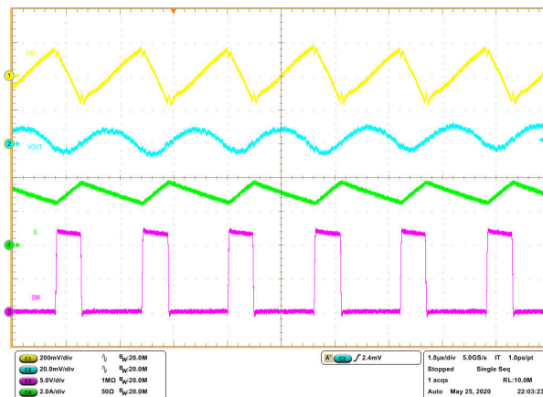
图 8-9. Steady State Waveforms, I_{OUT} = 3\text{ A}
