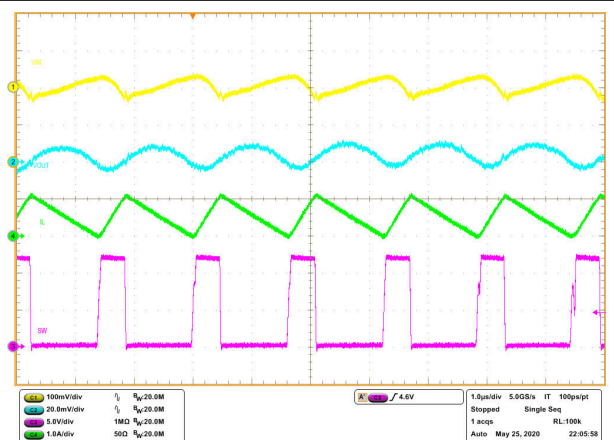
8-7. Steady State Waveforms, I_{OUT} = 0.5\text{ A}
