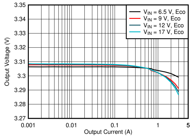
8-3. Load Regulation
