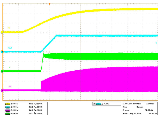
图 8-16. Start-Up Relative to VIN
