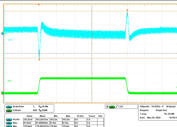
图 8-11. Transient Response 0 to 3 A with Slew Rate of 0.25\text{ A}/\mu\text{s} (FCCM)
