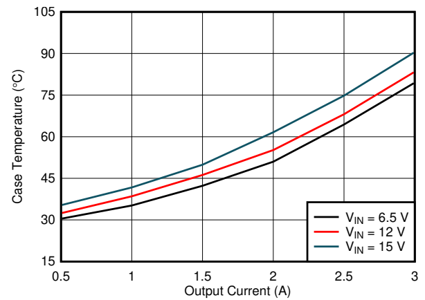
8-5. Case Temperature Rise vs Load Current
