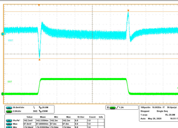
图 8-13. Transient Response 0.03 to 3 A with Slew Rate of 0.25\text{ A}/\mu\text{s} (FCCM)
