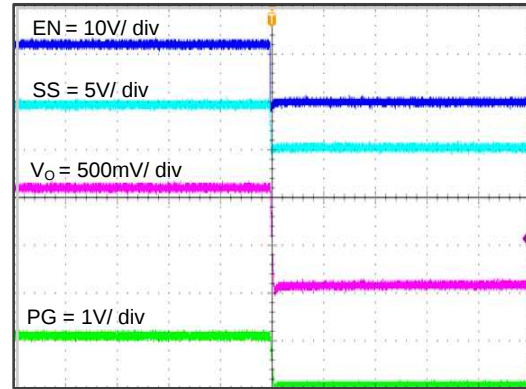
FIG 31. TPS562210A Shut Down Relative To EN
