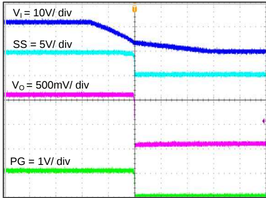
FIG 30. TPS562210A Shut Down Relative To V_I
