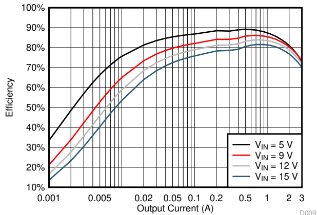
図 5-9. TPS563201 V_{OUT} = 1.05\text{ V} Efficiency, L = 2.2\text{ }\mu\text{H}
