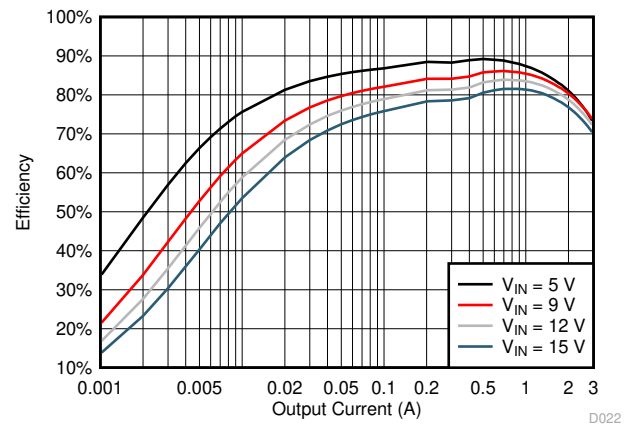
Figure 7-5. TPS563201 Efficiency
