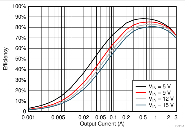
図 5-14. TPS563208 V_{OUT} = 1.05\text{ V} Efficiency, L = 2.2\text{ }\mu\text{H}
