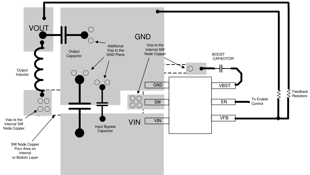
図 7-18. TPS563201 and TPS563208 Layout
