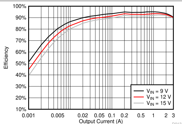
図 5-13. TPS563201 V_{OUT} = 5\text{ V} Efficiency, L = 3.3\text{ }\mu\text{H}
