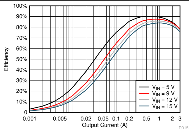
図 5-15. TPS563208 V_{OUT} = 1.5\text{ V} Efficiency, L = 2.2\text{ }\mu\text{H}
