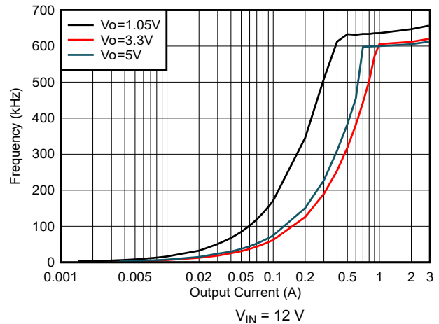
図 5-8. TPS563201 Switching Frequency vs Output Current
