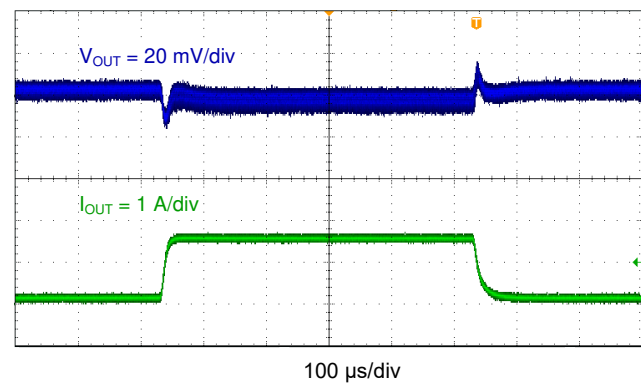
図 7-13. TPS563208 Transient Response 0.1 to 2 A
