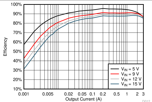
図 5-12. TPS563201 V_{OUT} = 3.3\text{ V} Efficiency, L = 2.2\text{ }\mu\text{H}
