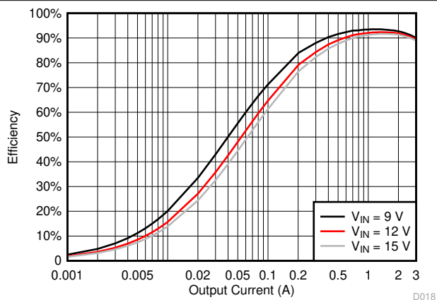
図 5-18. TPS563208 V_{OUT} = 5\text{ V} Efficiency, L = 3.3\text{ }\mu\text{H}
