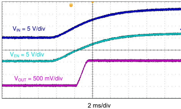
7-14. TPS563201 Start Up Relative to V_I
