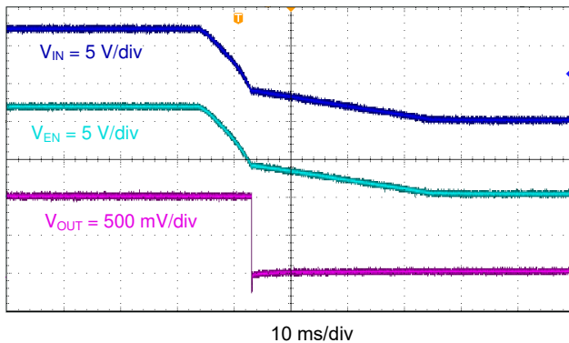
7-16. TPS563201 Shutdown Relative to V_I
