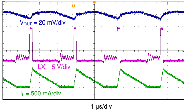
図 7-8. TPS563201 Output Voltage Ripple, I_{out} = 0.25 A
