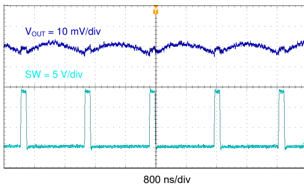
図 7-10. TPS563208 Output Voltage Ripple, I_{OUT} = 0 A
