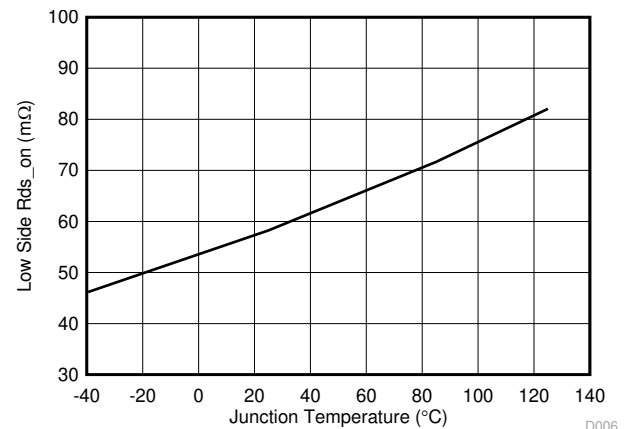
Figure 5-6. Low-Side R_{ds-On} vs Junction Temperature
