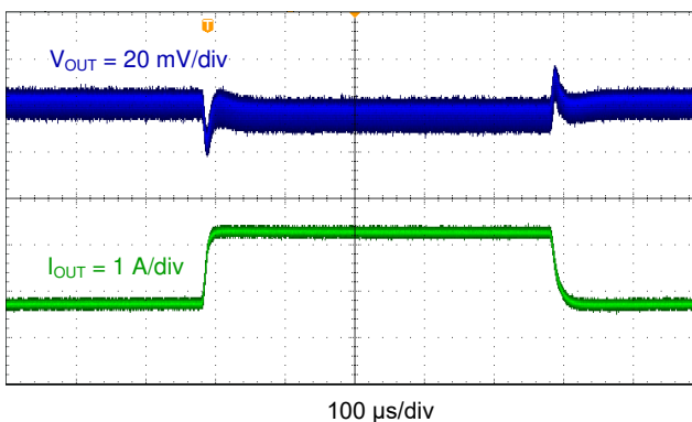
図 7-12. TPS563201 Transient Response, 0.75 to 2.25 A
