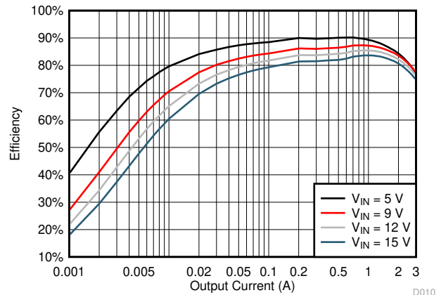
図 5-10. TPS563201 V_{OUT} = 1.5\text{ V} Efficiency, L = 2.2\text{ }\mu\text{H}
