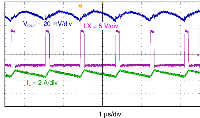
図 7-9. TPS563201 Output Voltage Ripple, I_{out} = 2 A
