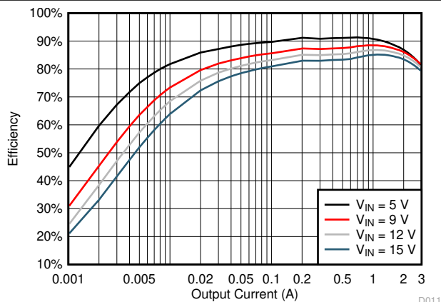
図 5-11. TPS563201 V_{OUT} = 1.8\text{ V} Efficiency, L = 2.2\text{ }\mu\text{H}
