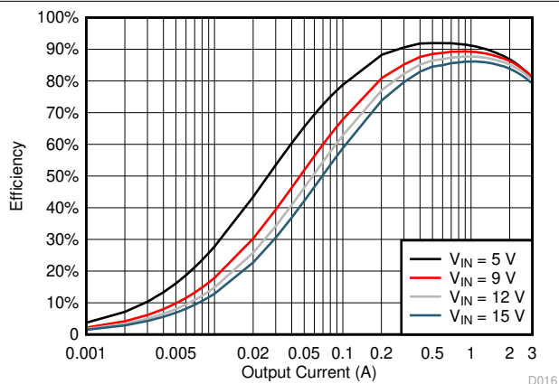
図 5-16. TPS563208 V_{OUT} = 1.8\text{ V} Efficiency, L = 2.2\text{ }\mu\text{H}
