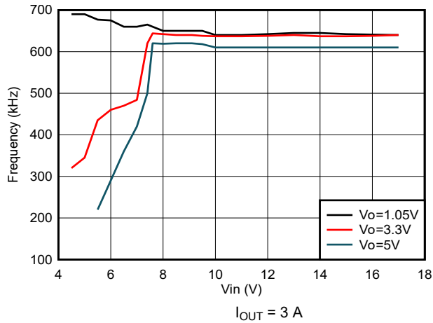
図 5-7. TPS563208 Switching Frequency vs Input Voltage
