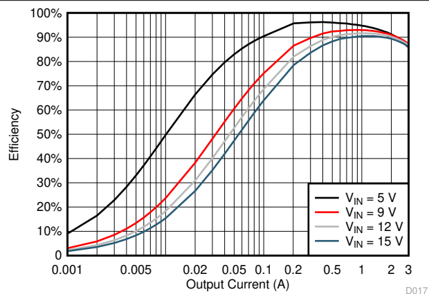
図 5-17. TPS563208 V_{OUT} = 3.3\text{ V} Efficiency, L = 2.2\text{ }\mu\text{H}
