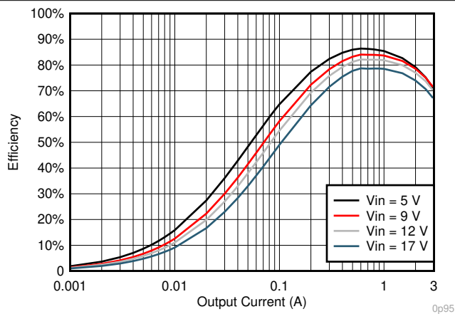
7-9. V_{OUT} = 0.95\text{-V} Efficiency, L = 1.5\text{ }\mu\text{H}
