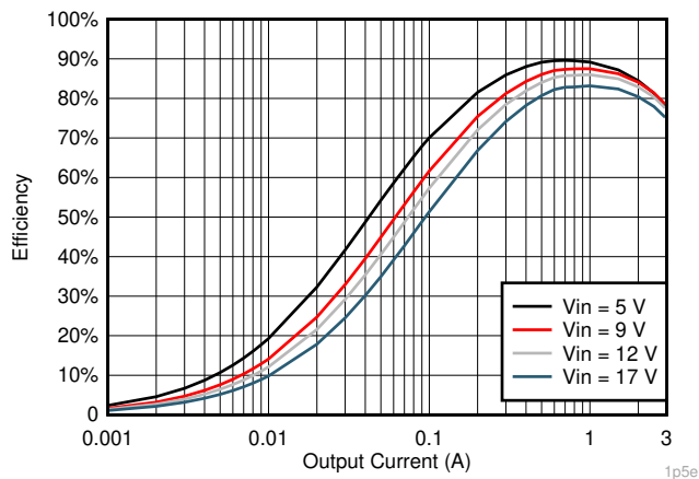
7-11. V_{OUT} = 1.5\text{-V} Efficiency, L = 2.2\text{ }\mu\text{H}
