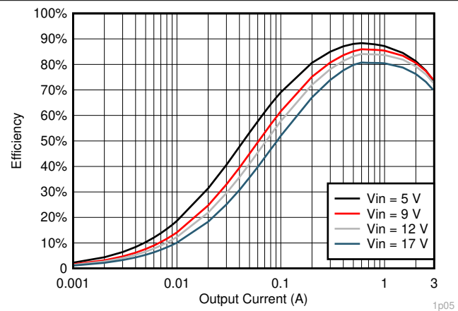
7-10. V_{OUT} = 1.05\text{-V} Efficiency, L = 1.5\text{ }\mu\text{H}
