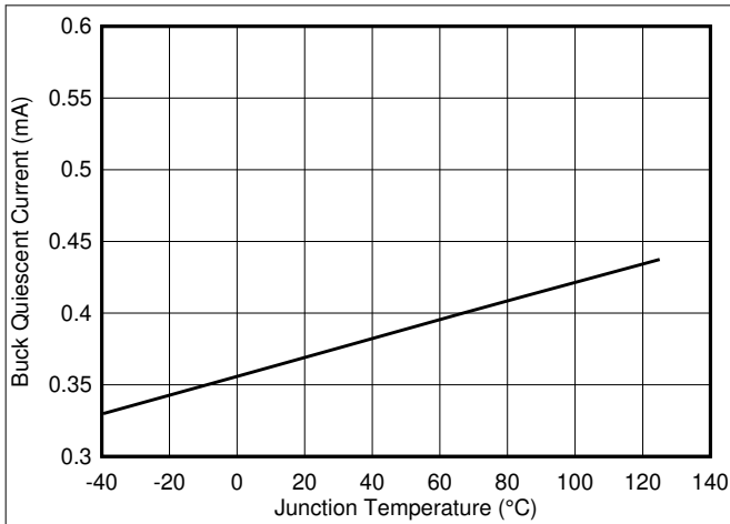
FIG 6-1. Supply Current vs Junction Temperature
