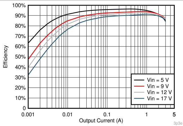
6-13. V_{OUT} = 3.3\text{ V} Efficiency, L = 3.3\text{ }\mu\text{H}
