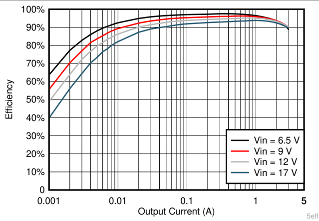
6-14. V_{OUT} = 5\text{ V} Efficiency, L = 4.7\text{ }\mu\text{H}
