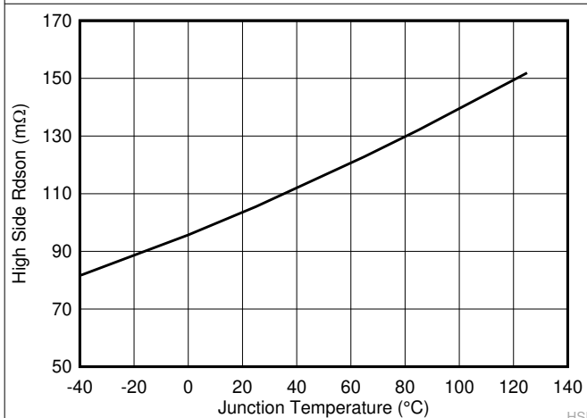
FIG 6-5. High-Side R_{ds-On} vs Junction Temperature
