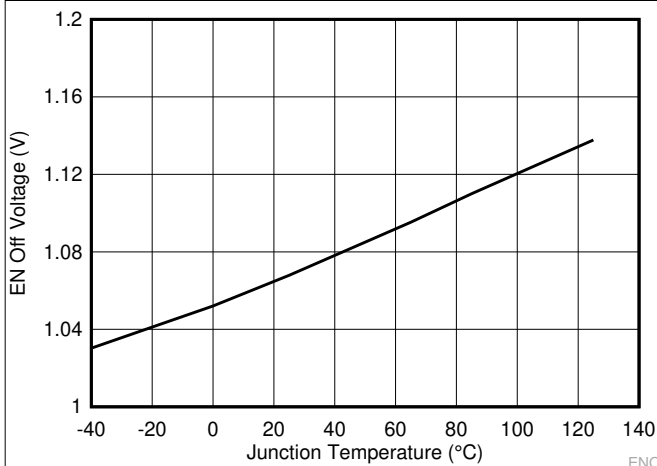
FIG 6-3. EN Pin EN Off Voltage vs Junction Temperature
