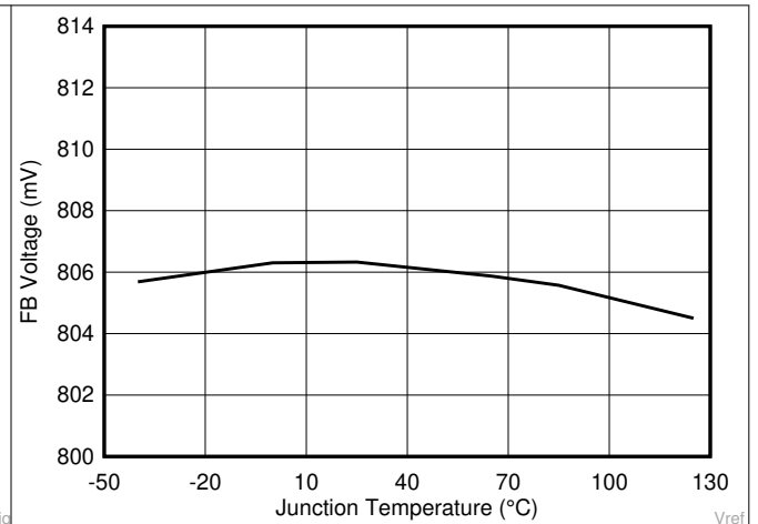
FIG 6-2. FB Voltage vs Junction Temperature
