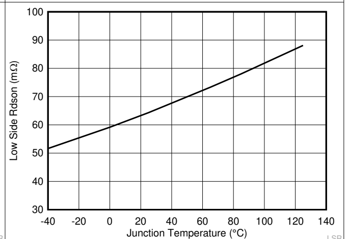
FIG 6-6. Low-Side R_{ds-On} vs Junction Temperature
