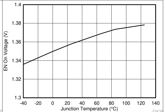
FIG 6-4. EN Pin EN On Voltage vs Junction Temperature
