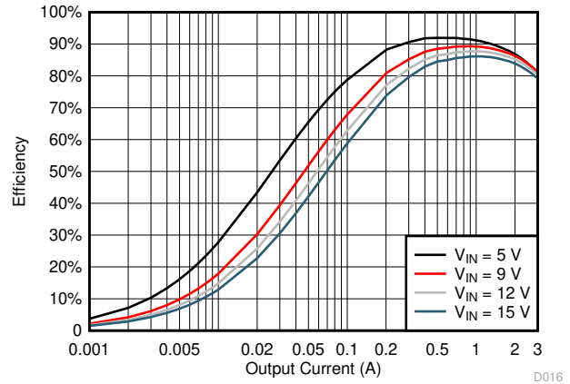
図 5-16. TPS563208 V_{OUT} = 1.8\text{ V} Efficiency, L = 2.2\text{ }\mu\text{H}
