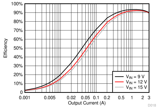
図 5-18. TPS563208 V_{OUT} = 5\text{ V} Efficiency, L = 3.3\text{ }\mu\text{H}
