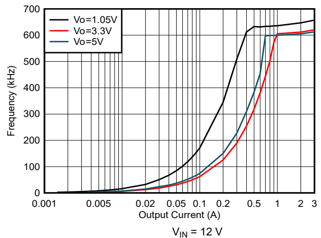
図 5-8. TPS563201 Switching Frequency vs Output Current
