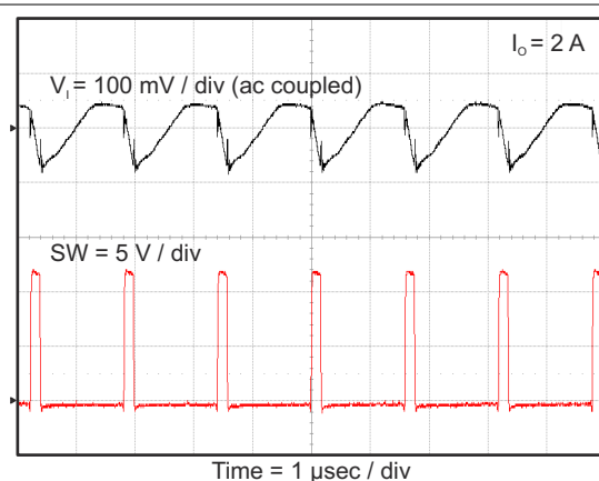
Figure 8-7. Tps562200 Input Voltage Ripple
