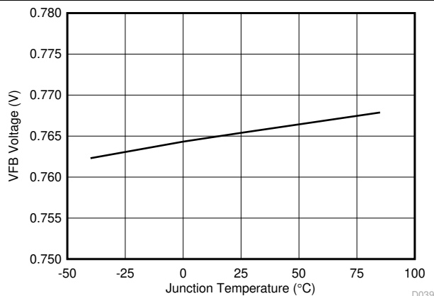
Figure 6-12. Vfb Voltage vs Junction Temperature
