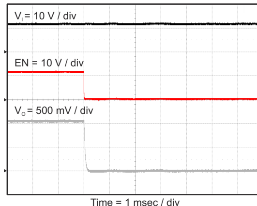
Figure 8-30. Tps563200 Shutdown Relative to EN
