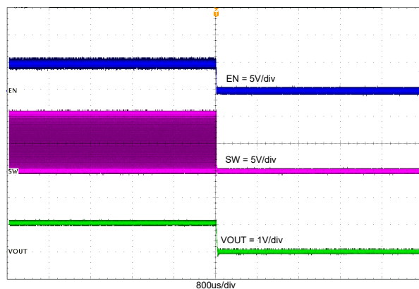
図 7-9. TPS562246 Enable Off With 2A Loading
