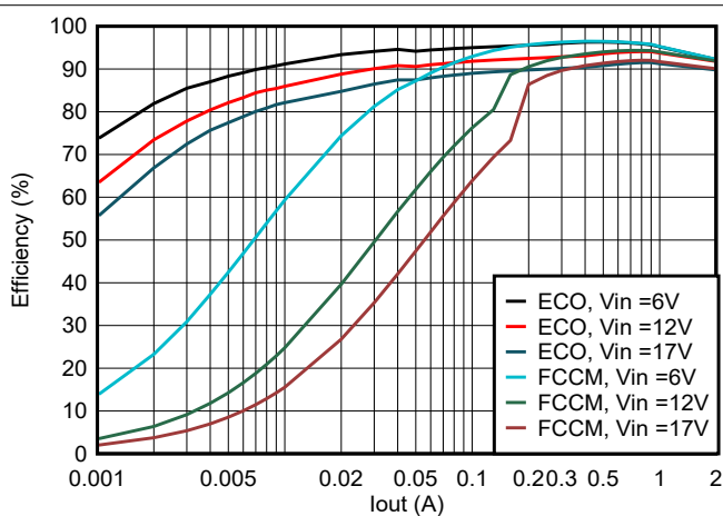
図 5-11. TPS56224x Efficiency at 3.3 Vout With 2.2uH Inductor
