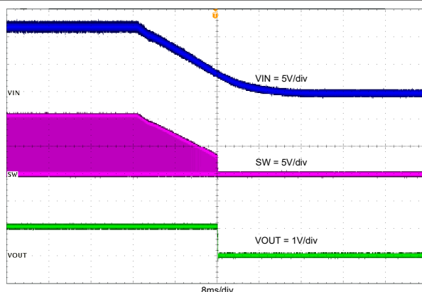
図 7-13. TPS562246 Power Off With 2A Loading
