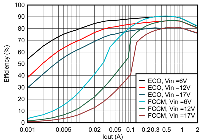
図 5-10. TPS56224x Efficiency at 1.05 Vout With 1.2uH Inductor
