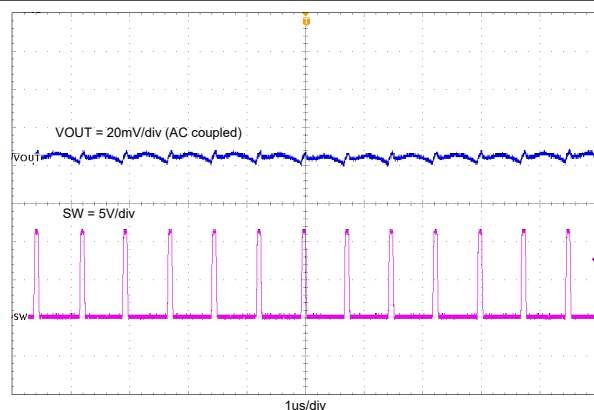
図 7-5. TPS562246 Output Voltage Ripple With 2A Loading
