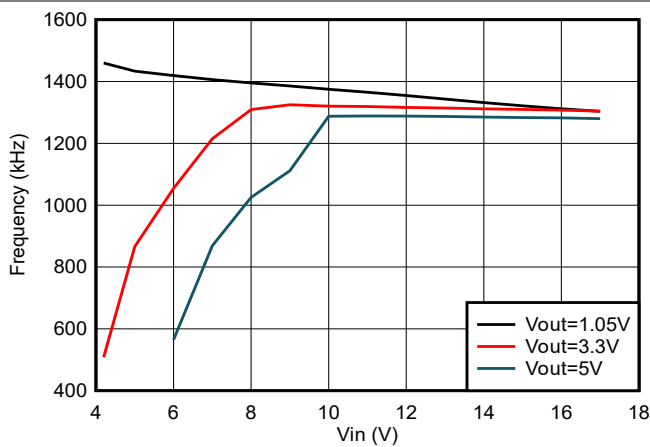
図 5-7. Frequency vs Input Voltage at 2A Loading
