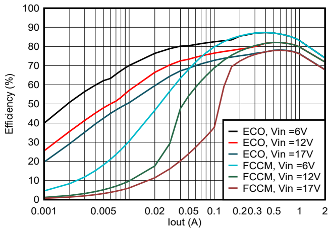
図 5-9. TPS56224x Efficiency at 0.6 Vout With 1uH Inductor
