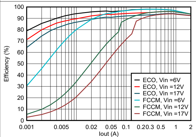
図 5-12. TPS56224x Efficiency at 5 Vout With 3.3uH Inductor
