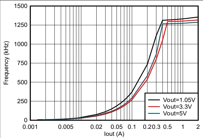
図 5-8. TPS562243 Frequency vs Loading
