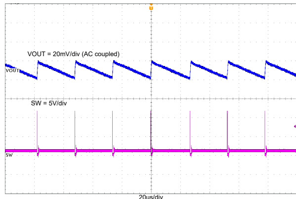
図 7-2. TPS562243 Output Voltage Ripple With 0.01A Loading
