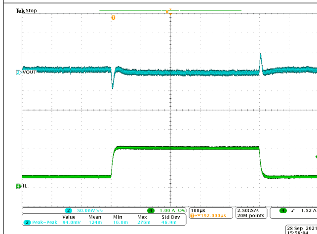
8-10. Transient Response 0.5 to 2 A with Slew Rate of 2.5\text{ A}/\mu\text{s}
