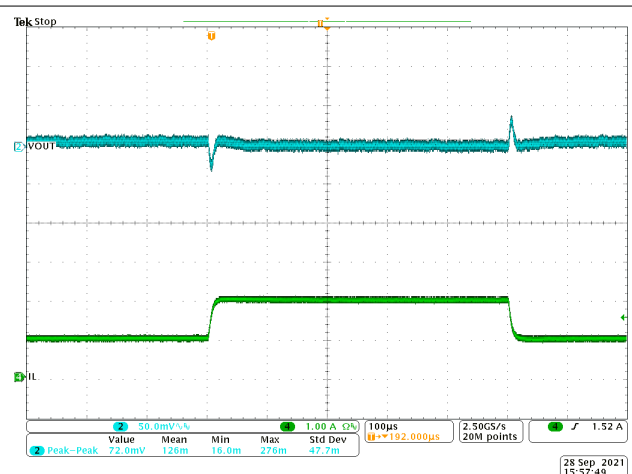
8-11. Transient Response 1 to 2 A with Slew Rate of 2.5\text{ A}/\mu\text{s}
