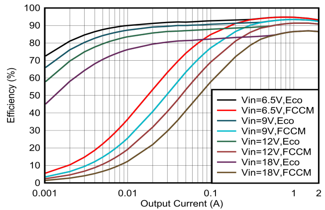
Figure 6-14. V_{OUT} = 3.3\text{-V} Efficiency, L = 2.2\text{ }\mu\text{H}
