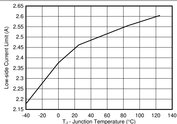
6-10. Low-Side Current Limit Threshold vs Junction Temperature
