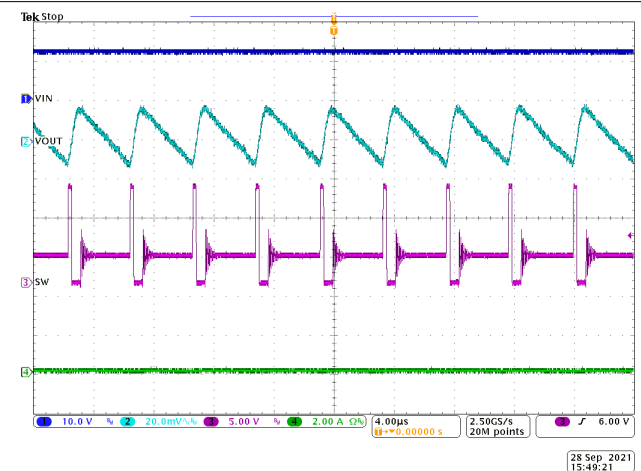
Figure 8-7. Steady State Waveforms, I_{OUT} = 0.1\text{ A}
