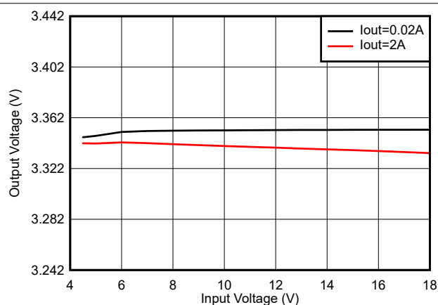
Figure 8-4. Line Regulation
