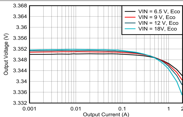
Figure 8-3. Load Regulation
