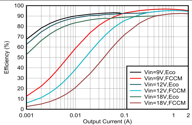
Figure 6-16. V_{OUT} = 7\text{-V} Efficiency, L = 3.3\text{ }\mu\text{H}
