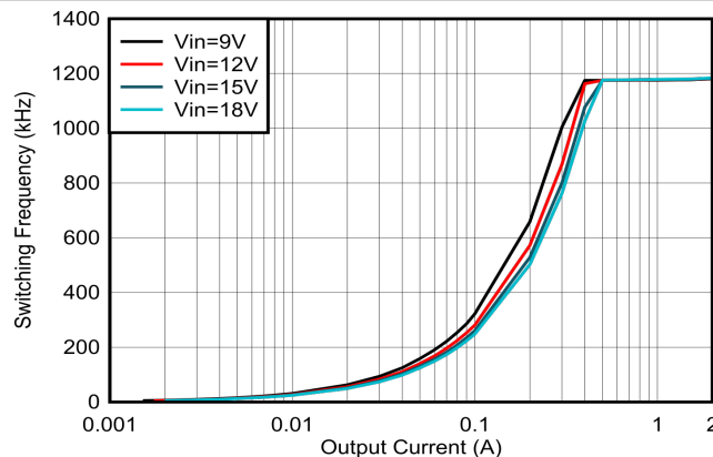
6-12. Switching Frequency vs Output Current, V_{OUT} = 3.3\text{ V} , L = 2.2\text{ }\mu\text{H}
