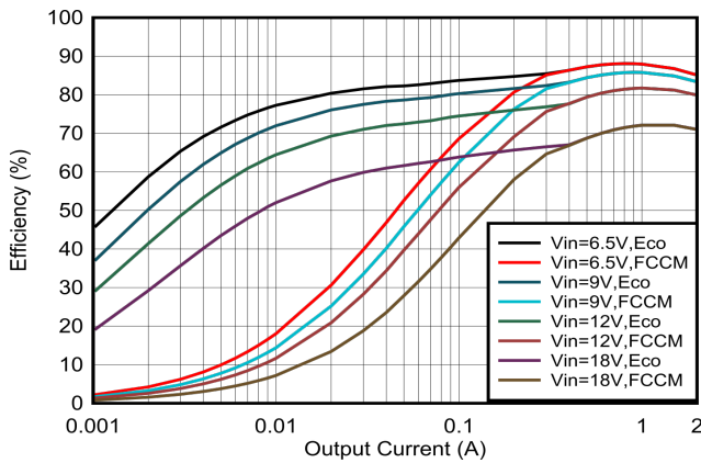
Figure 6-13. V_{OUT} = 1.05\text{-V} Efficiency, L = 1.0\text{ }\mu\text{H}
