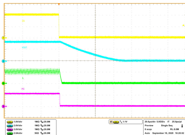
8-17. Disable Relative to EN
