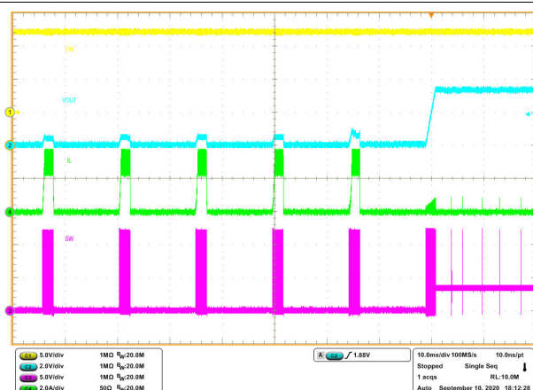
8-19. Output Short Recovery (ECO)
