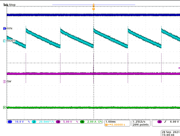
Figure 8-6. Steady State Waveforms, I_{OUT} = 0\text{ A}
