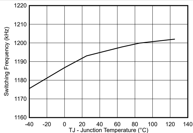
6-11. Switching Frequency vs Junction Temperature
