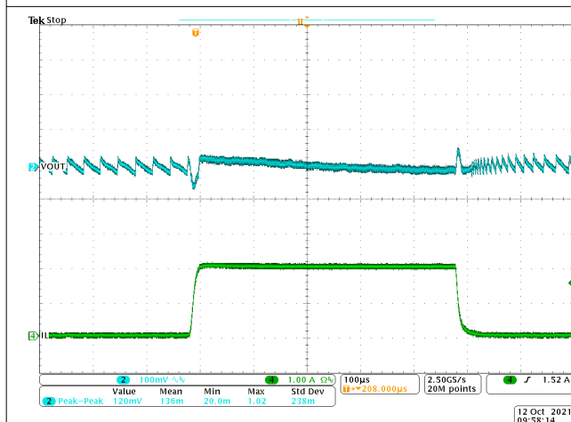
8-12. Transient Response 0 to 2 A with Slew Rate of 2.5\text{ A}/\mu\text{s} (ECO)
