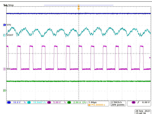
8-9. Steady State Waveforms, I_{OUT} = 2\text{ A}
