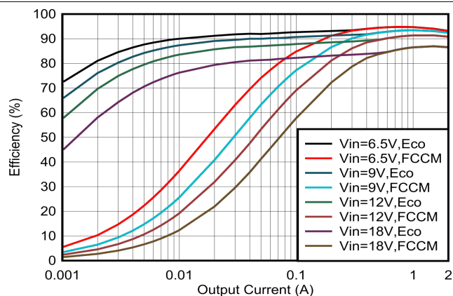
Figure 8-2. Efficiency
