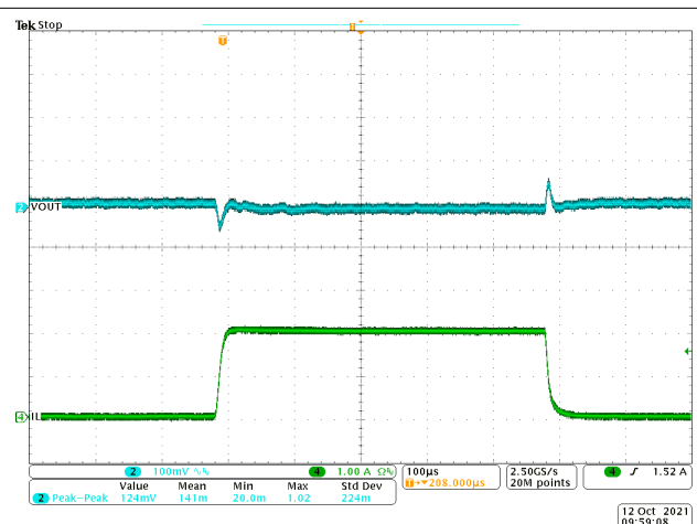
8-13. Transient Response 0 to 2 A with Slew Rate of 2.5\text{ A}/\mu\text{s} (FCCM)
