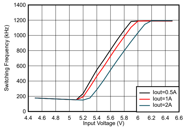
FIG 7-4. Frequency Foldback at Dropout ( V_{OUT} = 5\text{ V} )
