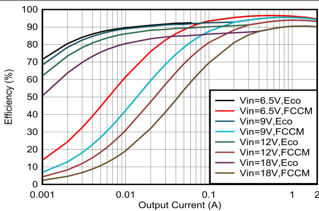
Figure 6-15. V_{OUT} = 5\text{-V} Efficiency, L = 3.3\text{ }\mu\text{H}
