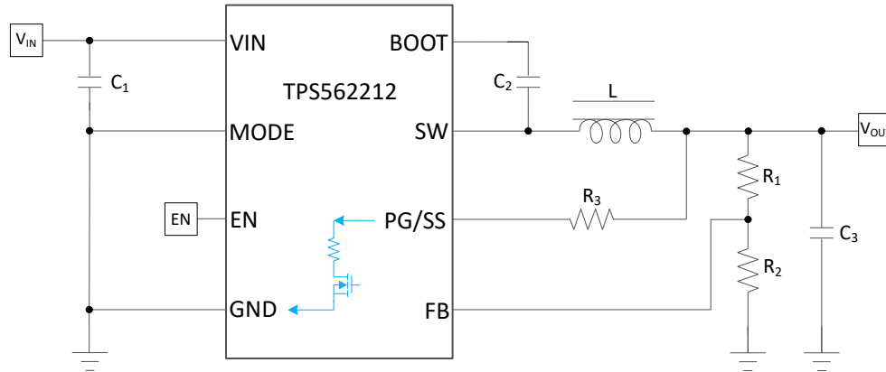
7-2. Discharge VOUT Through PG/SS Pin with TPS562212
