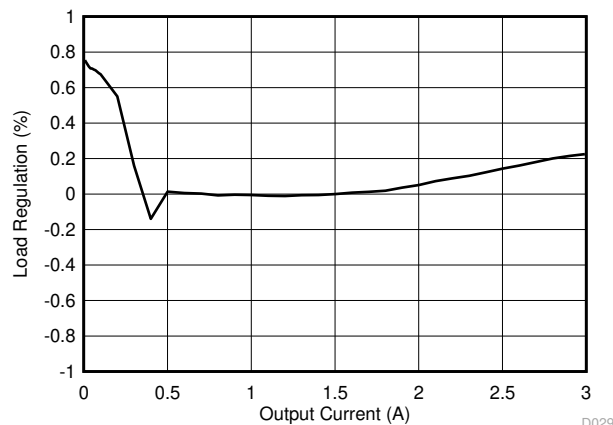
图 8-19. Tps563200 Load Regulation, V_I = 5V
