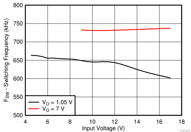
Figure 6-17. Switching Frequency vs Input Voltage
