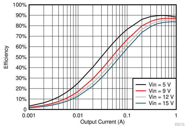
6-14. TPS561208 V_{OUT} = 1.5 V, Efficiency, L = 2.2 \mu H
