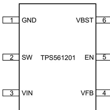
FIG 5-1. 6-Pin SOTDDC Package (Top View)
