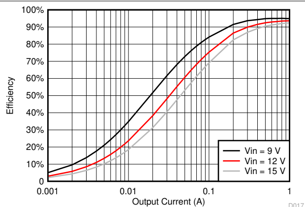
6-16. TPS561208 V_{OUT} = 5 V, Efficiency, L = 4.7 \mu H
