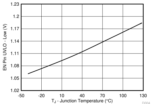
6-3. EN Pin UVLO Low Voltage vs Junction Temperature
