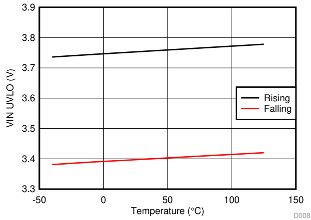
Figure 7. V_{IN} UVLO vs Temperature
